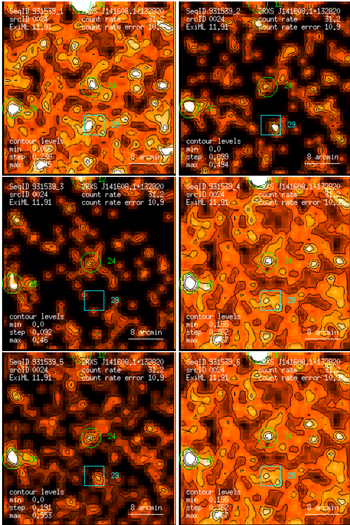
Figure 24: RASS 931539: detection 0024: band rate images, Gaussian filter: (1) PSPC channels 11 – 41, (2) 52 – 90, (3) 91 – 201, (4) 11 – 235, (5) 52 – 201, (6) 11 – 201. Broad band rates in counts/ks. Band rate contour levels in counts/ks/arcmin 2 .
