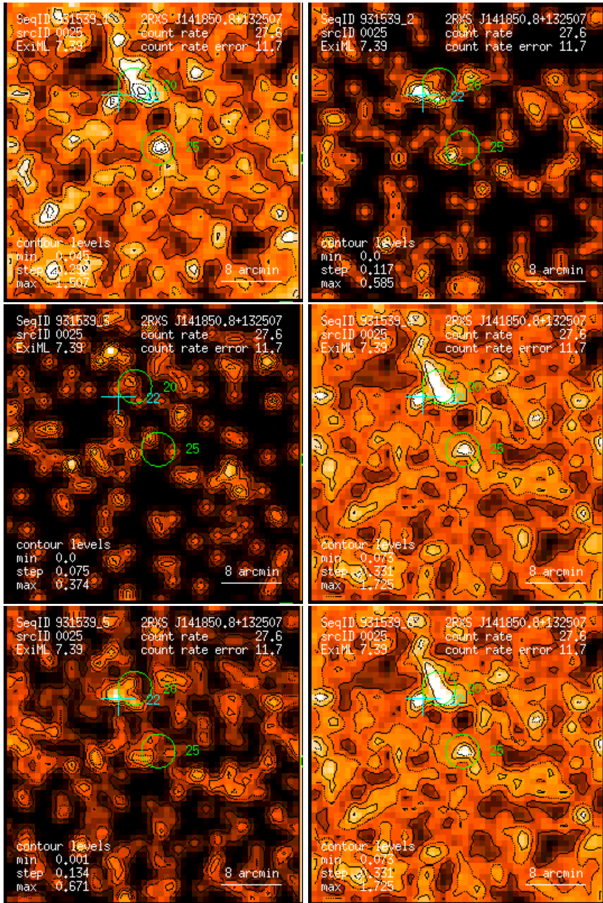
Figure 25: RASS 931539: detection 0025: band rate images, Gaussian filter: (1) PSPC channels 11 – 41, (2) 52 – 90, (3) 91 – 201, (4) 11 – 235, (5) 52 – 201, (6) 11 – 201. Broad band rates in counts/ks. Band rate contour levels in counts/ks/arcmin 2 .
