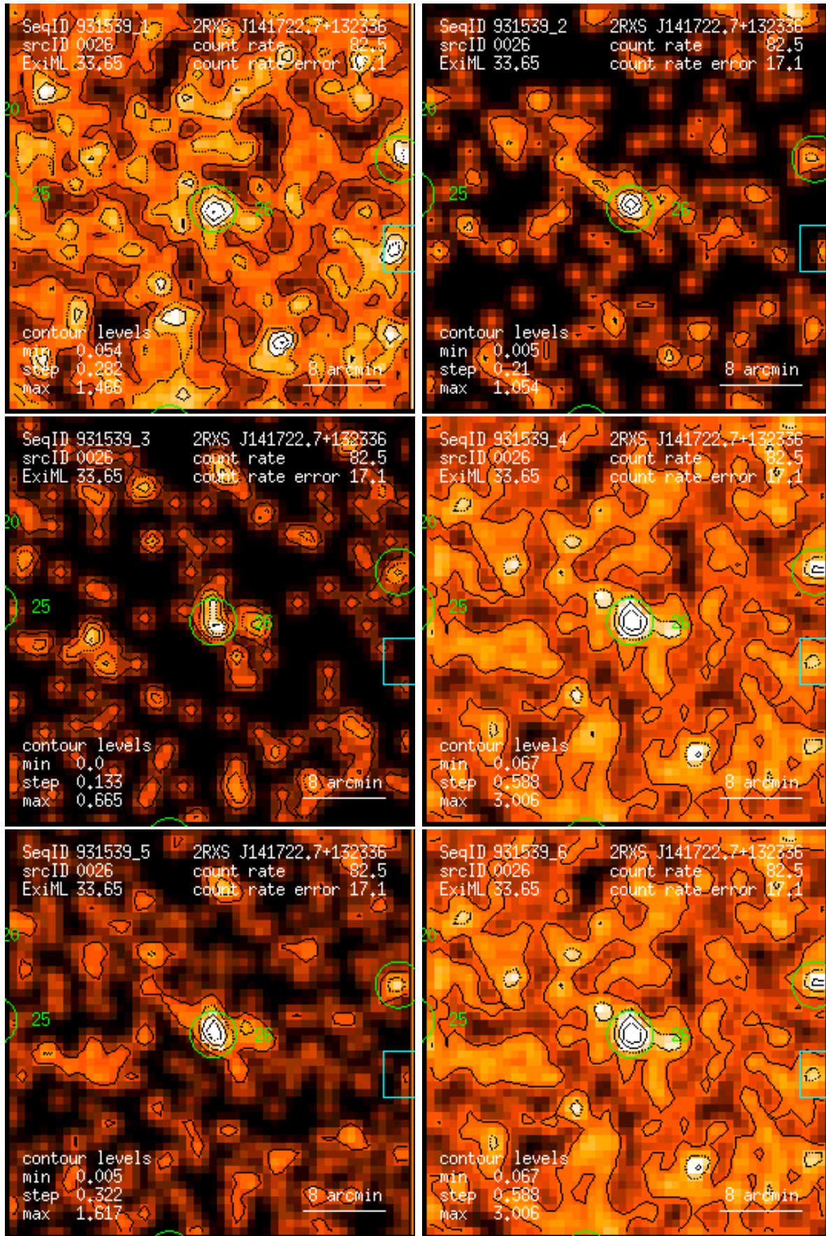
Figure 26: RASS 931539: detection 0026: band rate images, Gaussian filter: (1) PSPC channels 11 – 41, (2) 52 – 90, (3) 91 – 201, (4) 11 – 235, (5) 52 – 201, (6) 11 – 201. Broad band rates in counts/ks. Band rate contour levels in counts/ks/arcmin 2 .
