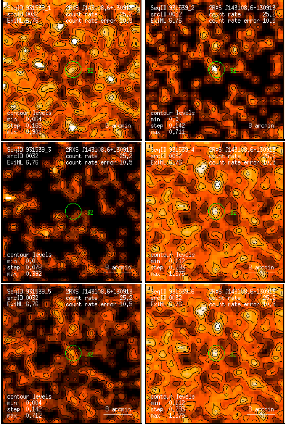
Figure 32: RASS 931539: detection 0032: band rate images, Gaussian filter: (1) PSPC channels 11 – 41, (2) 52 – 90, (3) 91 – 201, (4) 11 – 235, (5) 52 – 201, (6) 11 – 201. Broad band rates in counts/ks. Band rate contour levels in counts/ks/arcmin 2 .
