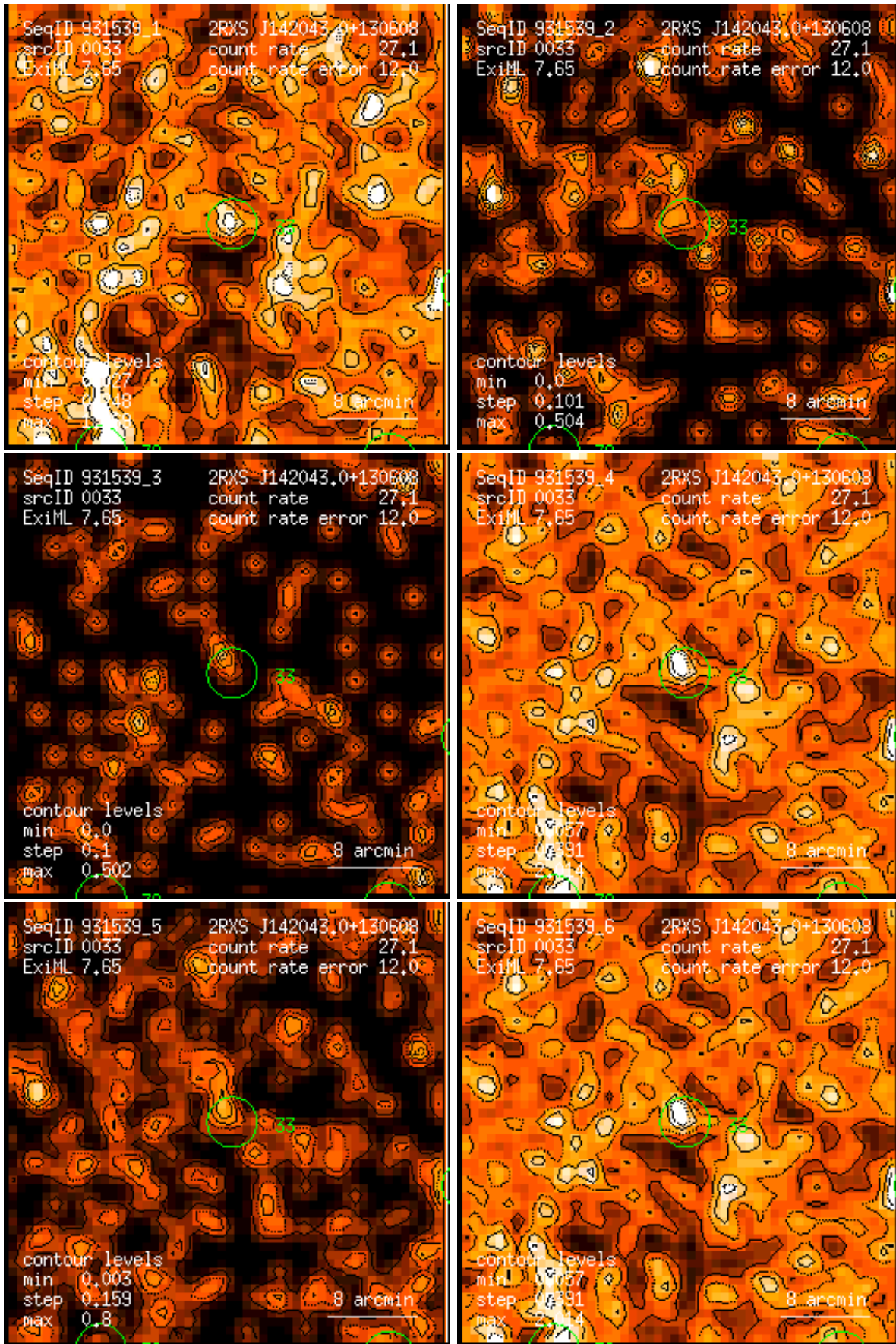
Figure 33: RASS 931539: detection 0033: band rate images, Gaussian filter: (1) PSPC channels 11 – 41, (2) 52 – 90, (3) 91 – 201, (4) 11 – 235, (5) 52 – 201, (6) 11 – 201. Broad band rates in counts/ks. Band rate contour levels in counts/ks/arcmin 2 .
