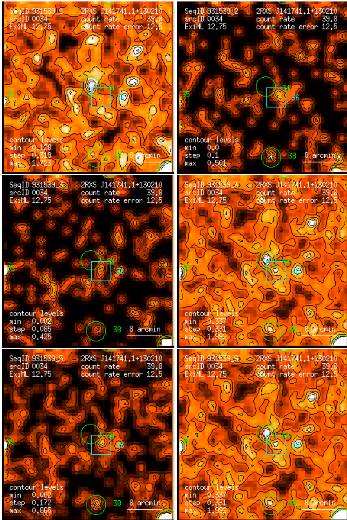
Figure 34: RASS 931539: detection 0034: band rate images, Gaussian filter: (1) PSPC channels 11 – 41, (2) 52 – 90, (3) 91 – 201, (4) 11 – 235, (5) 52 – 201, (6) 11 – 201. Broad band rates in counts/ks. Band rate contour levels in counts/ks/arcmin 2 .
