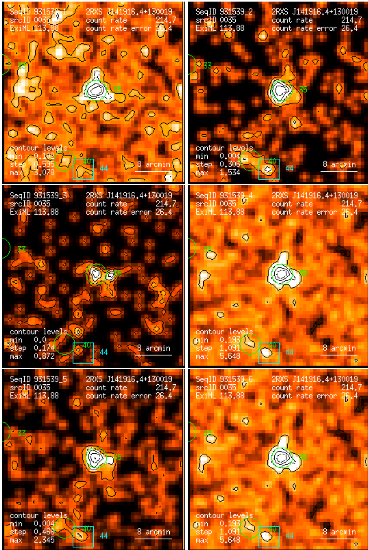
Figure 35: RASS 931539: detection 0035: band rate images, Gaussian filter: (1) PSPC channels 11 – 41, (2) 52 – 90, (3) 91 – 201, (4) 11 – 235, (5) 52 – 201, (6) 11 – 201. Broad band rates in counts/ks. Band rate contour levels in counts/ks/arcmin 2 .
