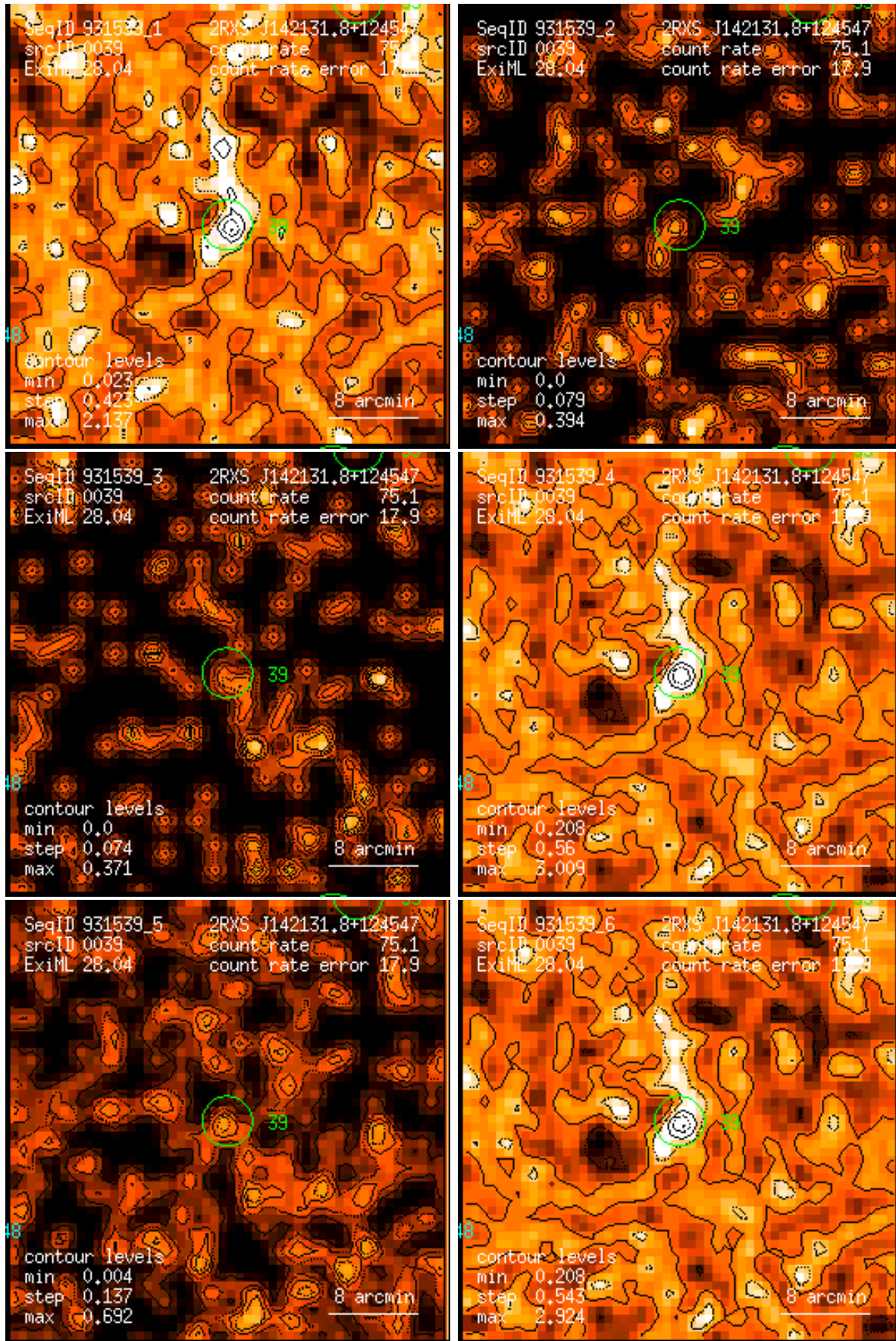
Figure 39: RASS 931539: detection 0039: band rate images, Gaussian filter: (1) PSPC channels 11 – 41, (2) 52 – 90, (3) 91 – 201, (4) 11 – 235, (5) 52 – 201, (6) 11 – 201. Broad band rates in counts/ks. Band rate contour levels in counts/ks/arcmin 2 .
