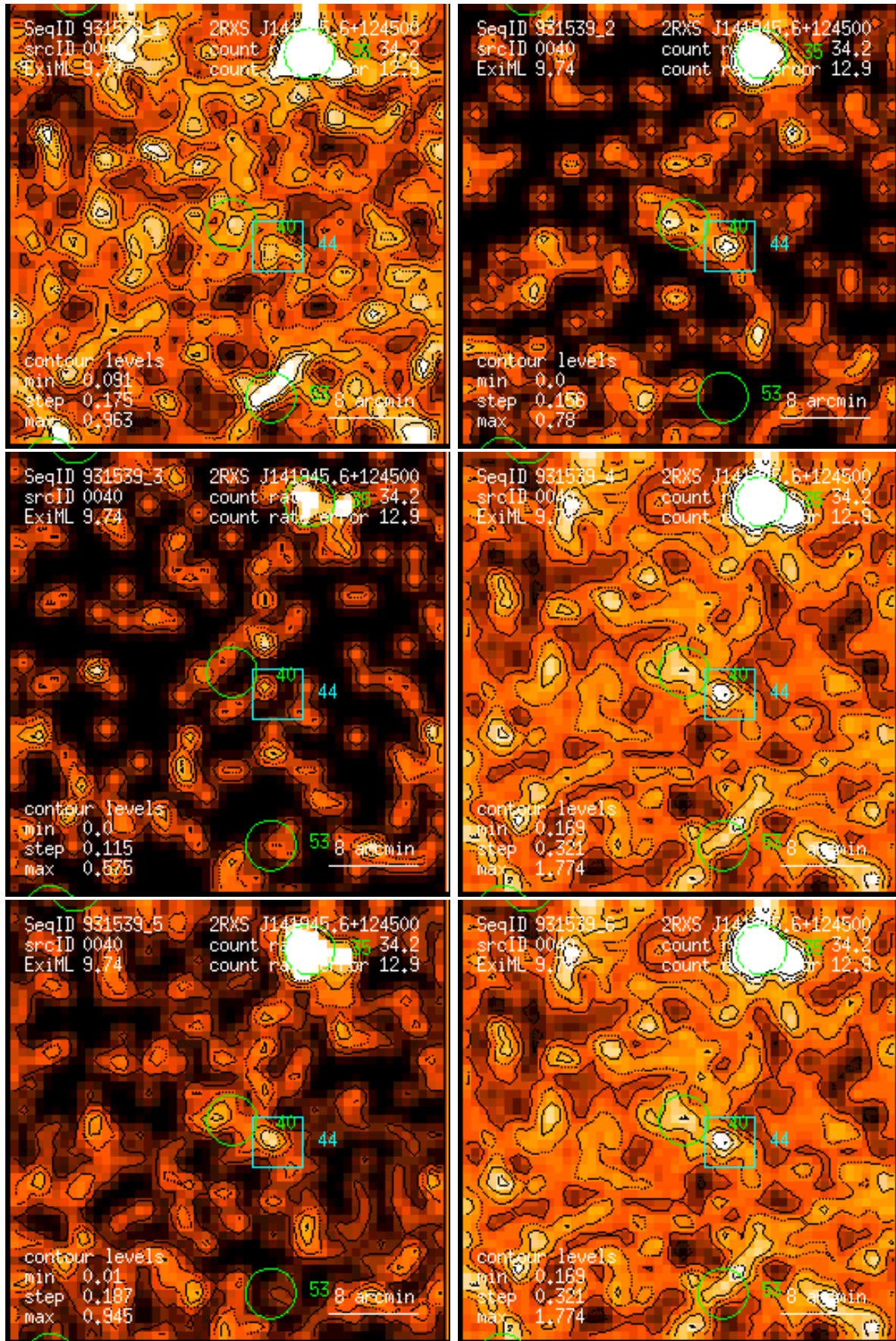
Figure 40: RASS 931539: detection 0040: band rate images, Gaussian filter: (1) PSPC channels 11 – 41, (2) 52 – 90, (3) 91 – 201, (4) 11 – 235, (5) 52 – 201, (6) 11 – 201. Broad band rates in counts/ks. Band rate contour levels in counts/ks/arcmin 2 .
