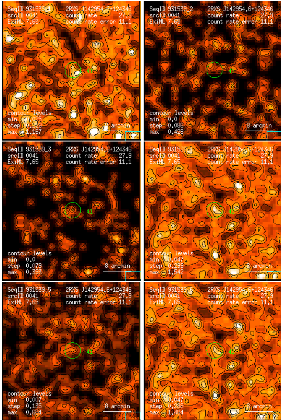
Figure 41: RASS 931539: detection 0041: band rate images, Gaussian filter: (1) PSPC channels 11 – 41, (2) 52 – 90, (3) 91 – 201, (4) 11 – 235, (5) 52 – 201, (6) 11 – 201. Broad band rates in counts/ks. Band rate contour levels in counts/ks/arcmin 2 .
