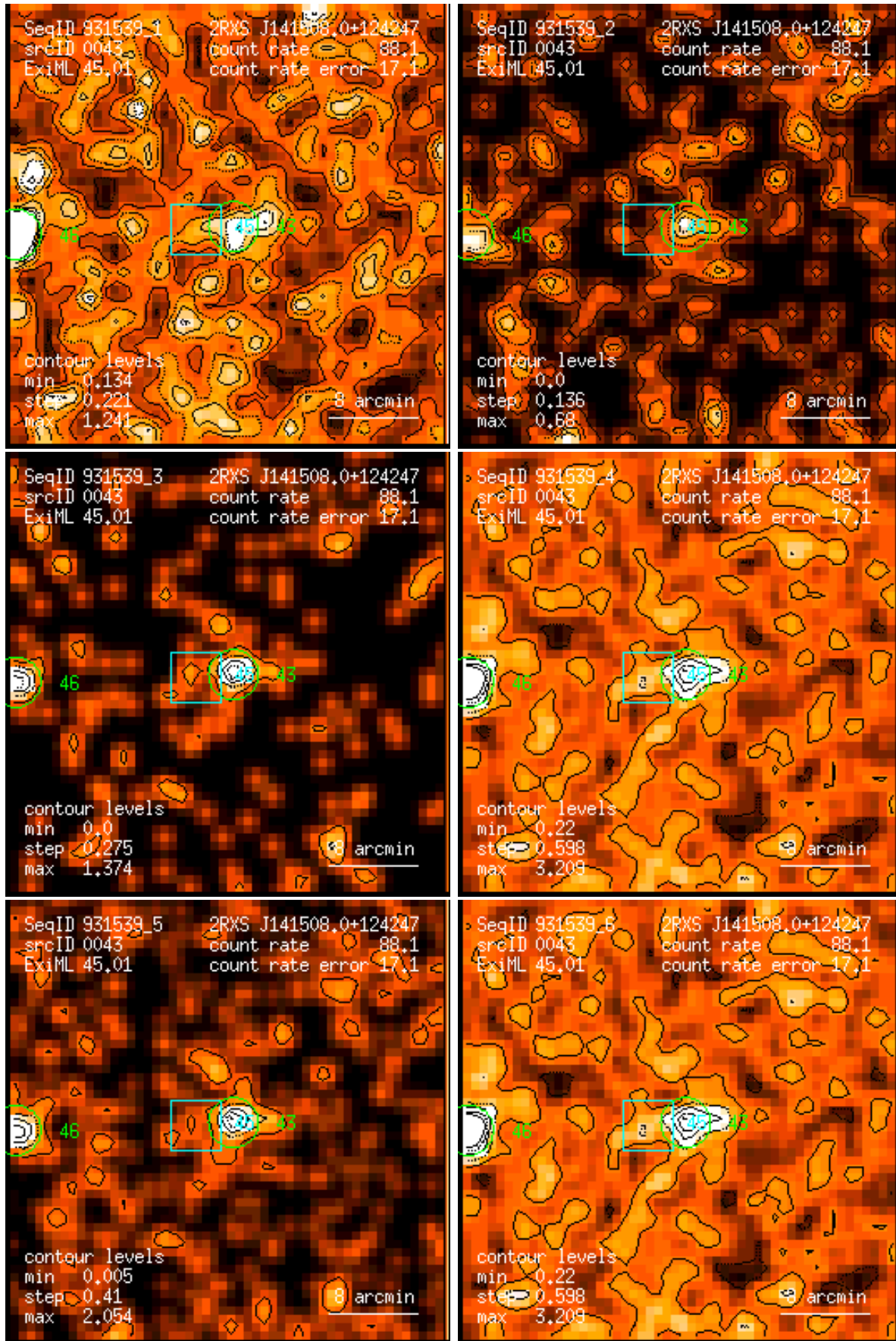
Figure 43: RASS 931539: detection 0043: band rate images, Gaussian filter: (1) PSPC channels 11 – 41, (2) 52 – 90, (3) 91 – 201, (4) 11 – 235, (5) 52 – 201, (6) 11 – 201. Broad band rates in counts/ks. Band rate contour levels in counts/ks/arcmin 2 .
