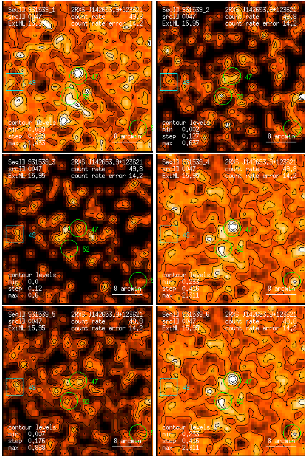
Figure 47: RASS 931539: detection 0047: band rate images, Gaussian filter: (1) PSPC channels 11 – 41, (2) 52 – 90, (3) 91 – 201, (4) 11 – 235, (5) 52 – 201, (6) 11 – 201. Broad band rates in counts/ks. Band rate contour levels in counts/ks/arcmin 2 .
