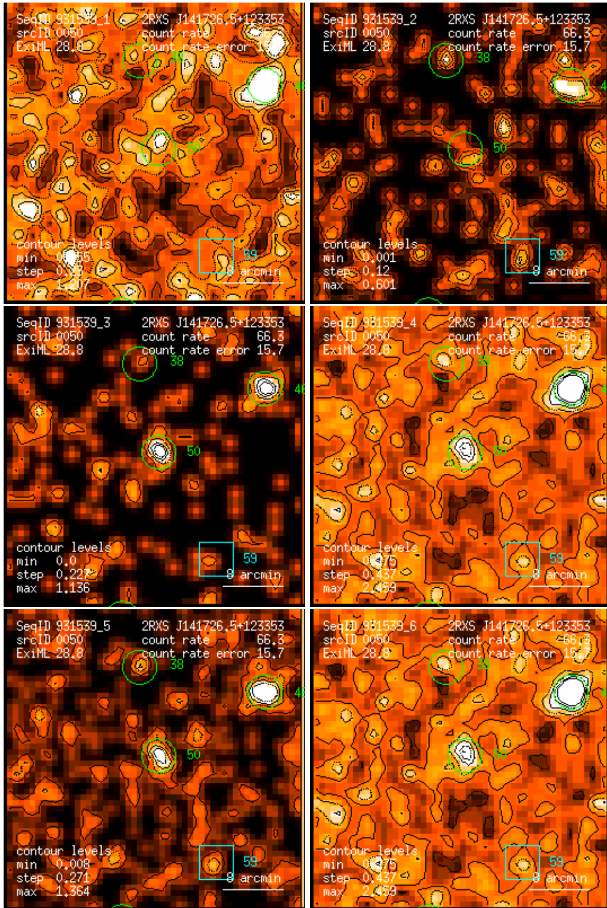
Figure 50: RASS 931539: detection 0050: band rate images, Gaussian filter: (1) PSPC channels 11 – 41, (2) 52 – 90, (3) 91 – 201, (4) 11 – 235, (5) 52 – 201, (6) 11 – 201. Broad band rates in counts/ks. Band rate contour levels in counts/ks/arcmin 2 .
