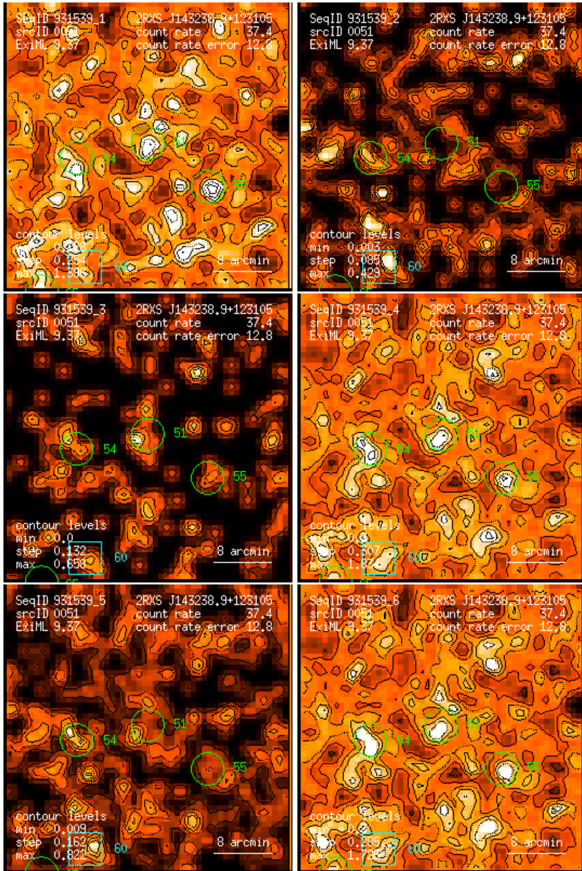
Figure 51: RASS 931539: detection 0051: band rate images, Gaussian filter: (1) PSPC channels 11 – 41, (2) 52 – 90, (3) 91 – 201, (4) 11 – 235, (5) 52 – 201, (6) 11 – 201. Broad band rates in counts/ks. Band rate contour levels in counts/ks/arcmin 2 .
