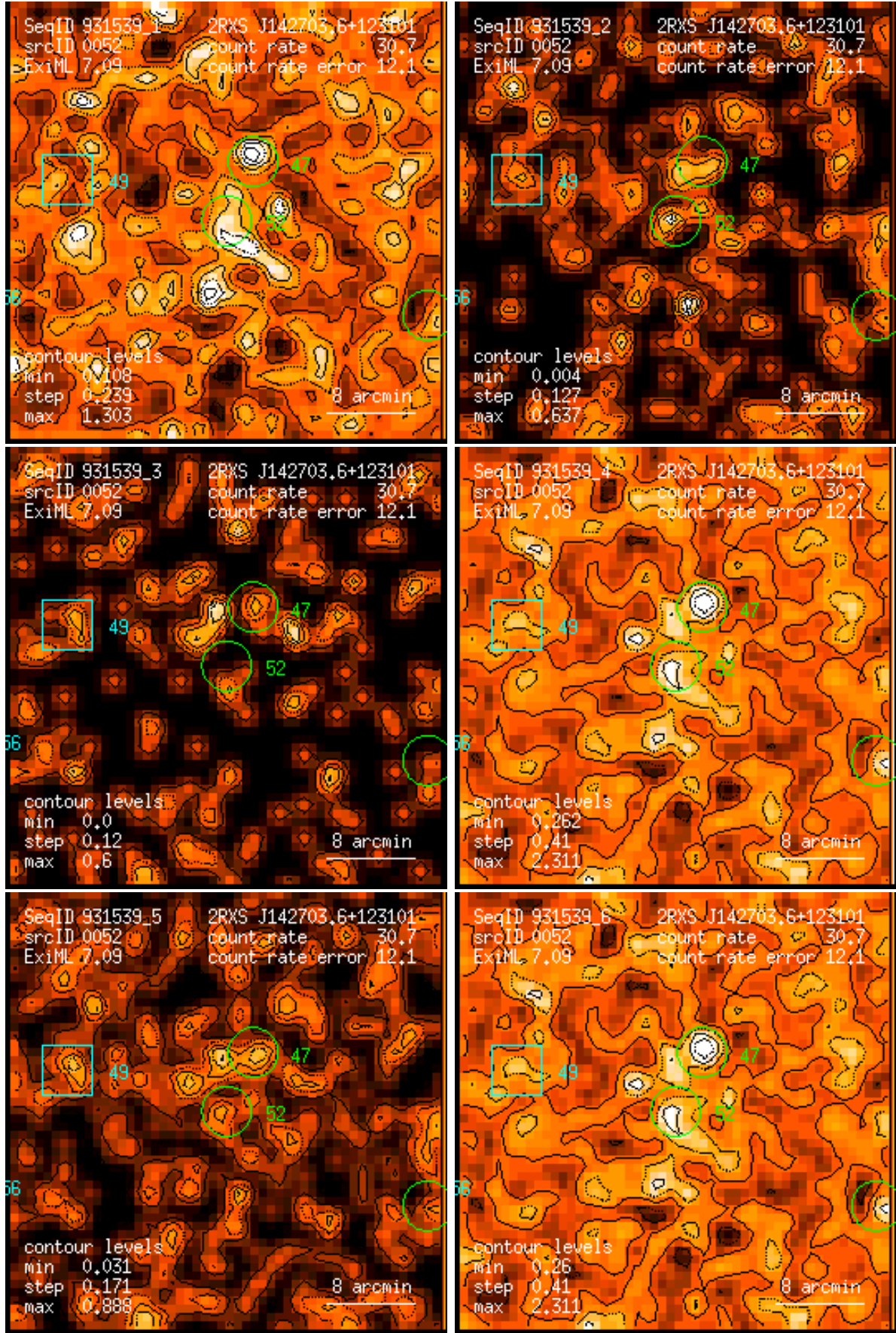
Figure 52: RASS 931539: detection 0052: band rate images, Gaussian filter: (1) PSPC channels 11 – 41, (2) 52 – 90, (3) 91 – 201, (4) 11 – 235, (5) 52 – 201, (6) 11 – 201. Broad band rates in counts/ks. Band rate contour levels in counts/ks/arcmin 2 .
