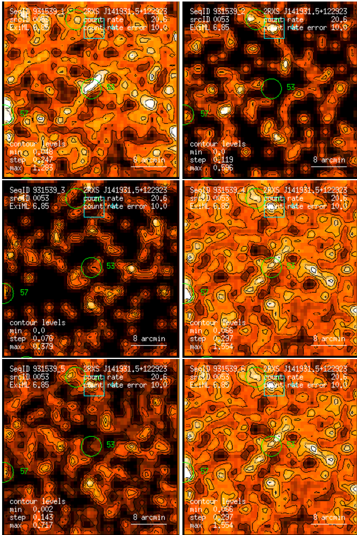
Figure 53: RASS 931539: detection 0053: band rate images, Gaussian filter: (1) PSPC channels 11 – 41, (2) 52 – 90, (3) 91 – 201, (4) 11 – 235, (5) 52 – 201, (6) 11 – 201. Broad band rates in counts/ks. Band rate contour levels in counts/ks/arcmin 2 .
