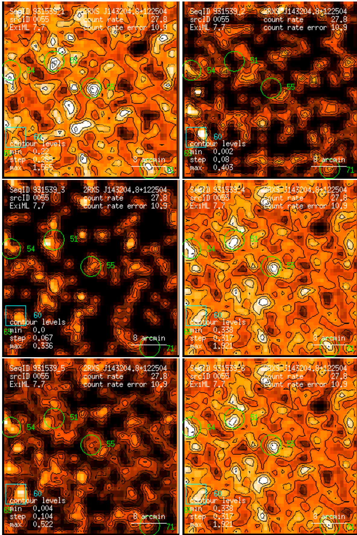
Figure 55: RASS 931539: detection 0055: band rate images, Gaussian filter: (1) PSPC channels 11 – 41, (2) 52 – 90, (3) 91 – 201, (4) 11 – 235, (5) 52 – 201, (6) 11 – 201. Broad band rates in counts/ks. Band rate contour levels in counts/ks/arcmin 2 .
