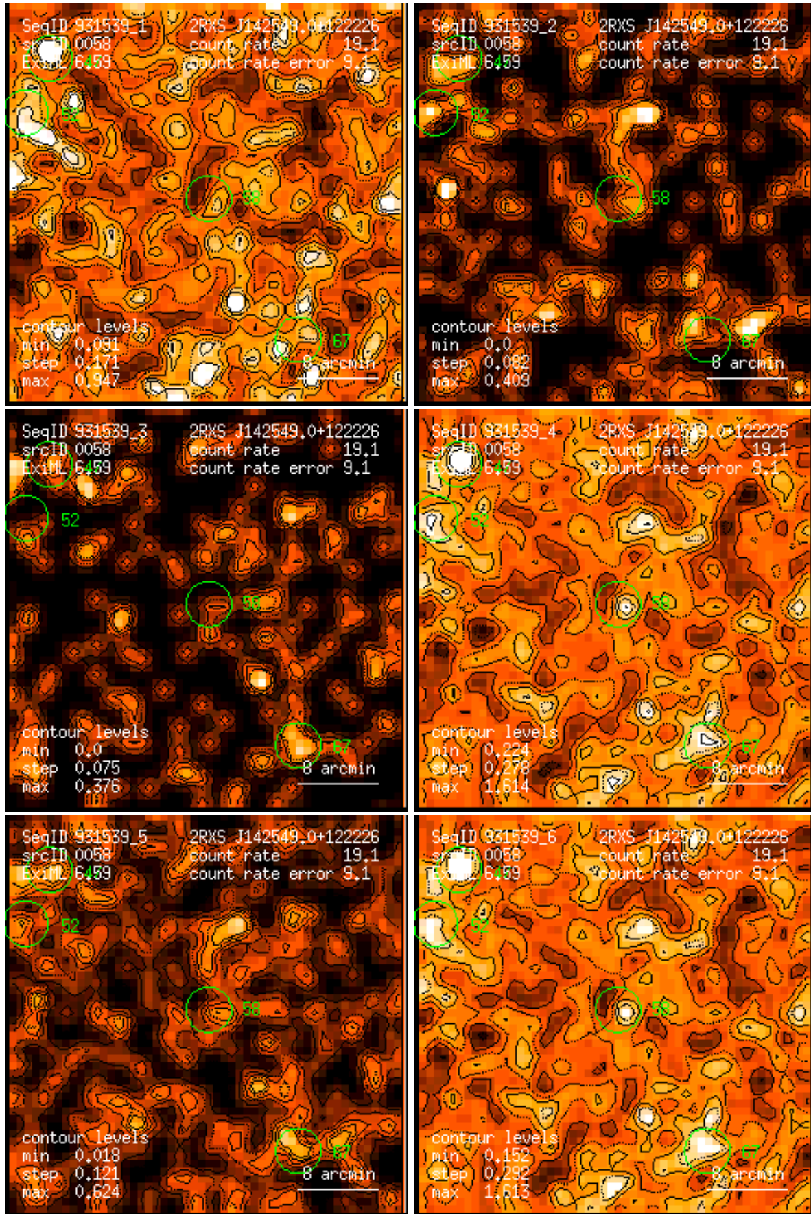
Figure 58: RASS 931539: detection 0058: band rate images, Gaussian filter: (1) PSPC channels 11 – 41, (2) 52 – 90, (3) 91 – 201, (4) 11 – 235, (5) 52 – 201, (6) 11 – 201. Broad band rates in counts/ks. Band rate contour levels in counts/ks/arcmin 2 .
