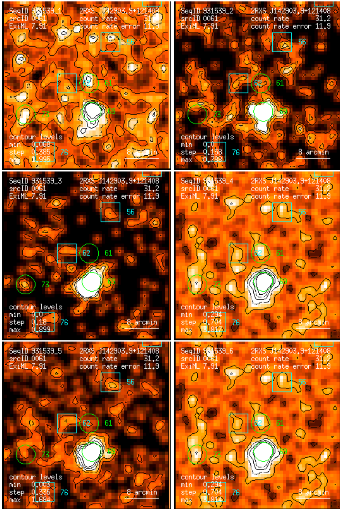
Figure 61: RASS 931539: detection 0061: band rate images, Gaussian filter: (1) PSPC channels 11 – 41, (2) 52 – 90, (3) 91 – 201, (4) 11 – 235, (5) 52 – 201, (6) 11 – 201. Broad band rates in counts/ks. Band rate contour levels in counts/ks/arcmin 2 .
