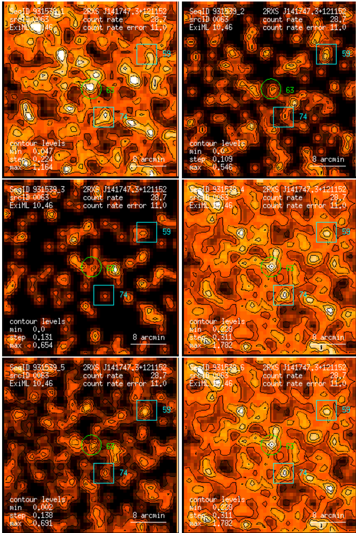
Figure 63: RASS 931539: detection 0063: band rate images, Gaussian filter: (1) PSPC channels 11 – 41, (2) 52 – 90, (3) 91 – 201, (4) 11 – 235, (5) 52 – 201, (6) 11 – 201. Broad band rates in counts/ks. Band rate contour levels in counts/ks/arcmin 2 .
