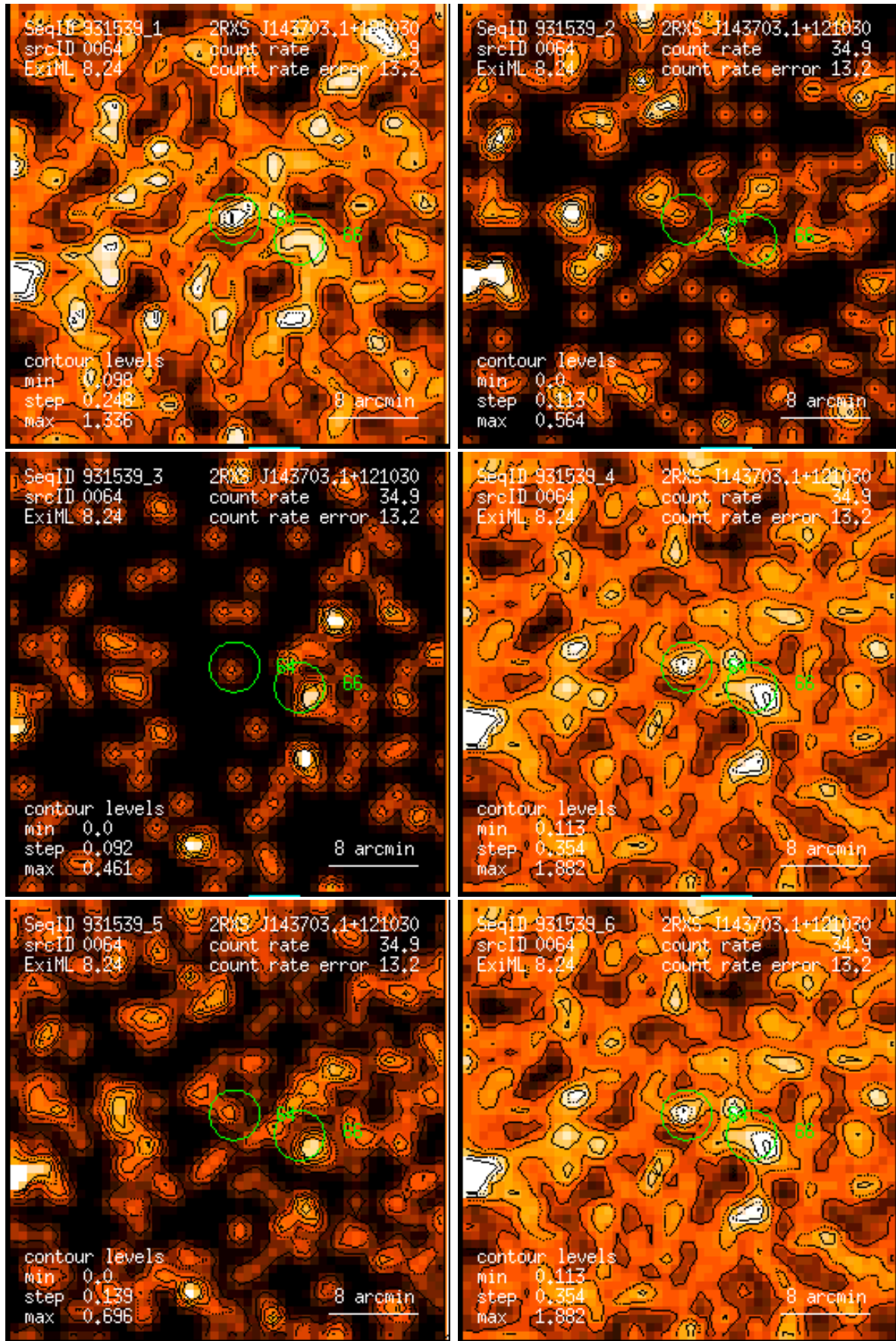
Figure 64: RASS 931539: detection 0064: band rate images, Gaussian filter: (1) PSPC channels 11 – 41, (2) 52 – 90, (3) 91 – 201, (4) 11 – 235, (5) 52 – 201, (6) 11 – 201. Broad band rates in counts/ks. Band rate contour levels in counts/ks/arcmin 2 .
