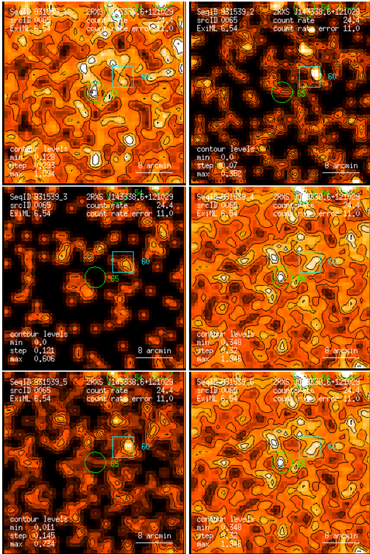
Figure 65: RASS 931539: detection 0065: band rate images, Gaussian filter: (1) PSPC channels 11 – 41, (2) 52 – 90, (3) 91 – 201, (4) 11 – 235, (5) 52 – 201, (6) 11 – 201. Broad band rates in counts/ks. Band rate contour levels in counts/ks/arcmin 2 .
