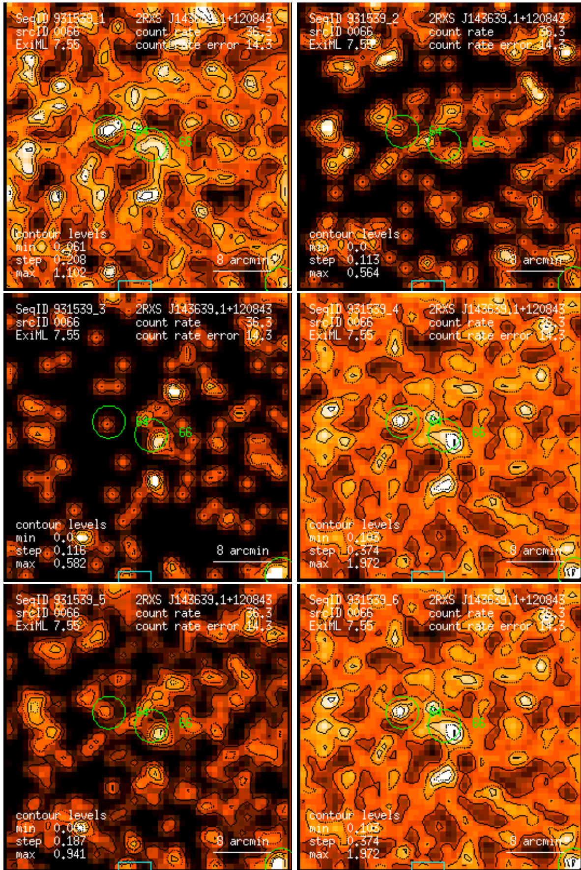
Figure 66: RASS 931539: detection 0066: band rate images, Gaussian filter: (1) PSPC channels 11 – 41, (2) 52 – 90, (3) 91 – 201, (4) 11 – 235, (5) 52 – 201, (6) 11 – 201. Broad band rates in counts/ks. Band rate contour levels in counts/ks/arcmin 2 .
