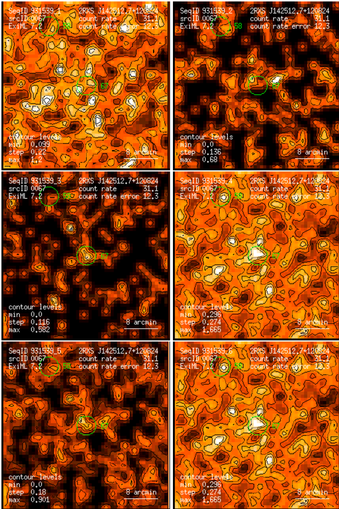
Figure 67: RASS 931539: detection 0067: band rate images, Gaussian filter: (1) PSPC channels 11 – 41, (2) 52 – 90, (3) 91 – 201, (4) 11 – 235, (5) 52 – 201, (6) 11 – 201. Broad band rates in counts/ks. Band rate contour levels in counts/ks/arcmin 2 .
