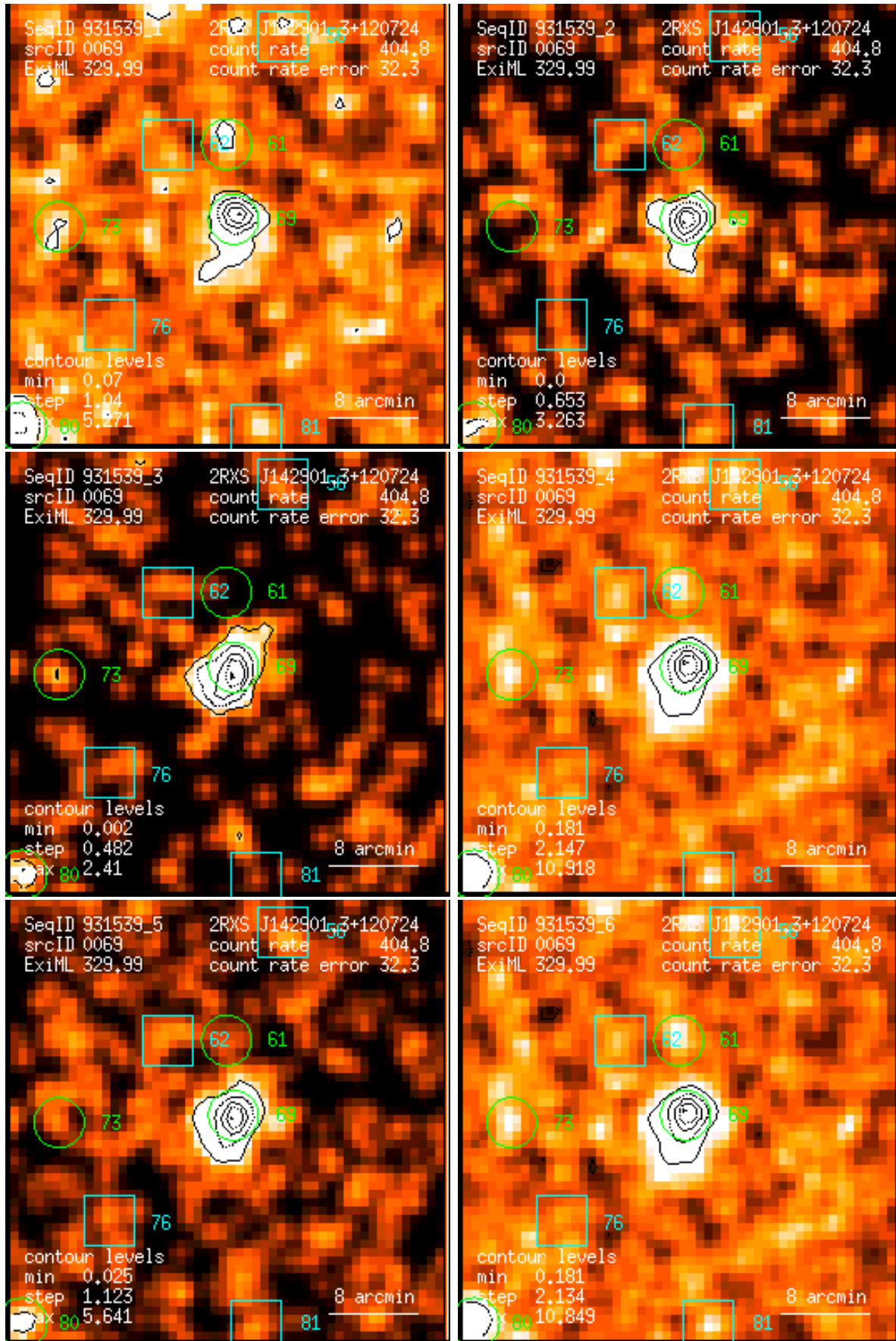
Figure 69: RASS 931539: detection 0069: band rate images, Gaussian filter: (1) PSPC channels 11 – 41, (2) 52 – 90, (3) 91 – 201, (4) 11 – 235, (5) 52 – 201, (6) 11 – 201. Broad band rates in counts/ks. Band rate contour levels in counts/ks/arcmin 2 .
