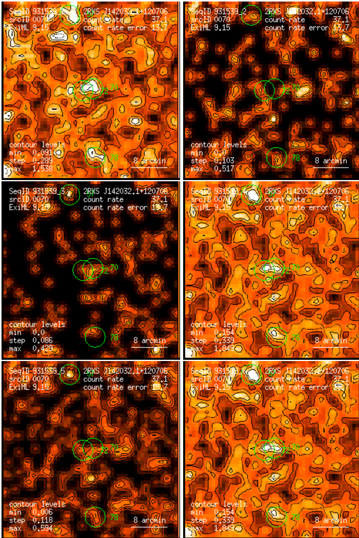
Figure 70: RASS 931539: detection 0070: band rate images, Gaussian filter: (1) PSPC channels 11 – 41, (2) 52 – 90, (3) 91 – 201, (4) 11 – 235, (5) 52 – 201, (6) 11 – 201. Broad band rates in counts/ks. Band rate contour levels in counts/ks/arcmin 2 .
