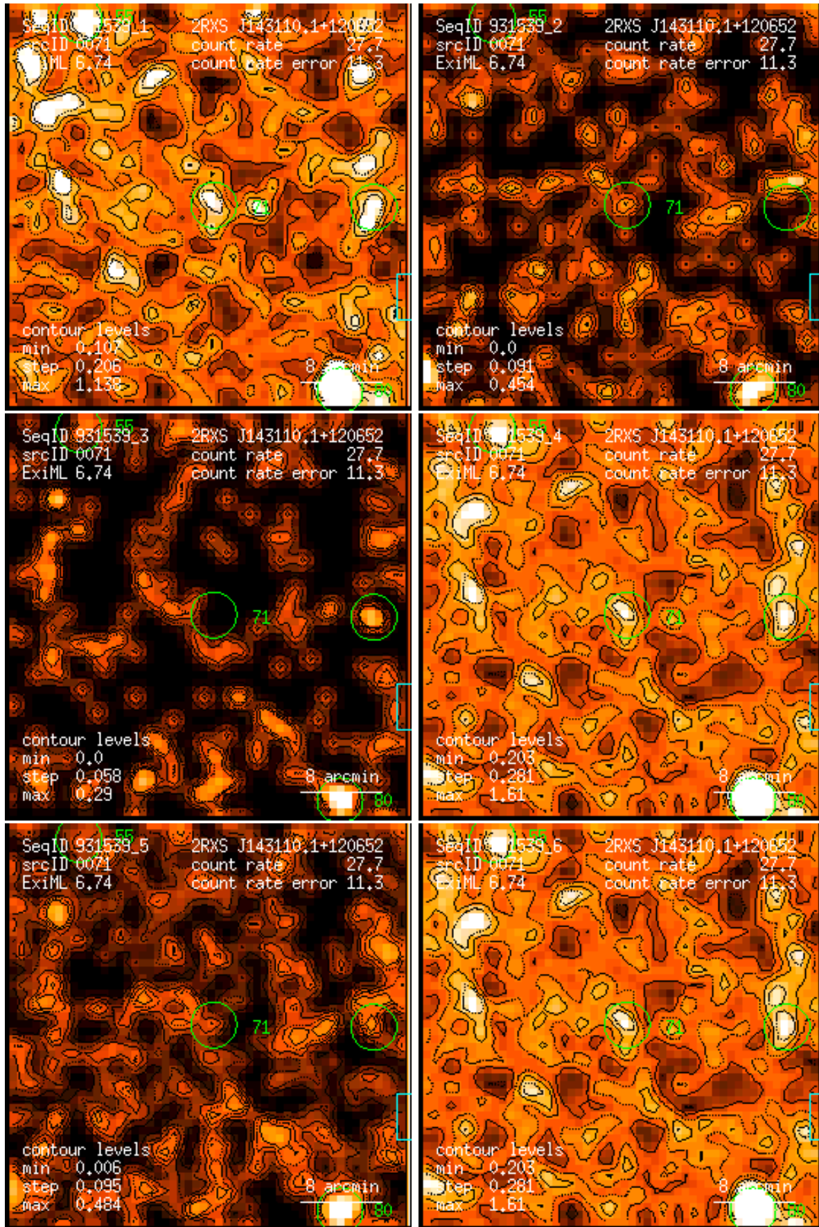
Figure 71: RASS 931539: detection 0071: band rate images, Gaussian filter: (1) PSPC channels 11 – 41, (2) 52 – 90, (3) 91 – 201, (4) 11 – 235, (5) 52 – 201, (6) 11 – 201. Broad band rates in counts/ks. Band rate contour levels in counts/ks/arcmin 2 .
