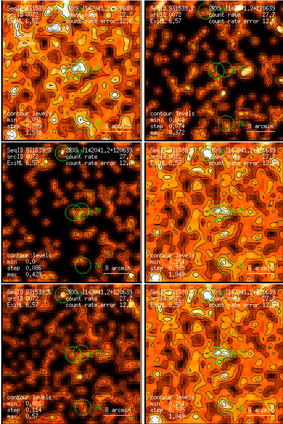
Figure 72: RASS 931539: detection 0072: band rate images, Gaussian filter: (1) PSPC channels 11 – 41, (2) 52 – 90, (3) 91 – 201, (4) 11 – 235, (5) 52 – 201, (6) 11 – 201. Broad band rates in counts/ks. Band rate contour levels in counts/ks/arcmin 2 .
