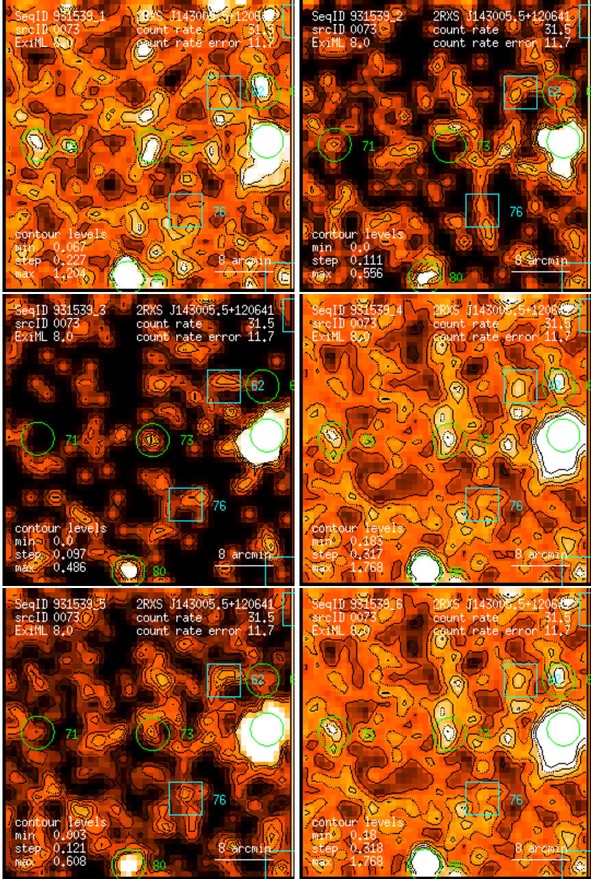
Figure 73: RASS 931539: detection 0073: band rate images, Gaussian filter: (1) PSPC channels 11 – 41, (2) 52 – 90, (3) 91 – 201, (4) 11 – 235, (5) 52 – 201, (6) 11 – 201. Broad band rates in counts/ks. Band rate contour levels in counts/ks/arcmin 2 .
