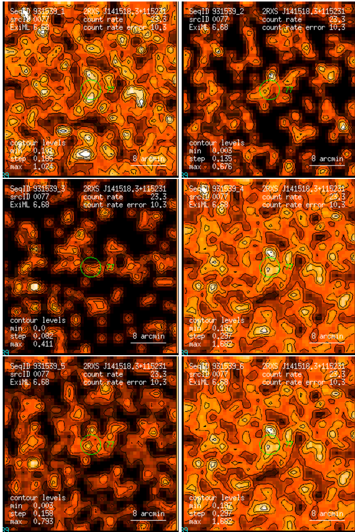
Figure 77: RASS 931539: detection 0077: band rate images, Gaussian filter: (1) PSPC channels 11 – 41, (2) 52 – 90, (3) 91 – 201, (4) 11 – 235, (5) 52 – 201, (6) 11 – 201. Broad band rates in counts/ks. Band rate contour levels in counts/ks/arcmin 2 .
