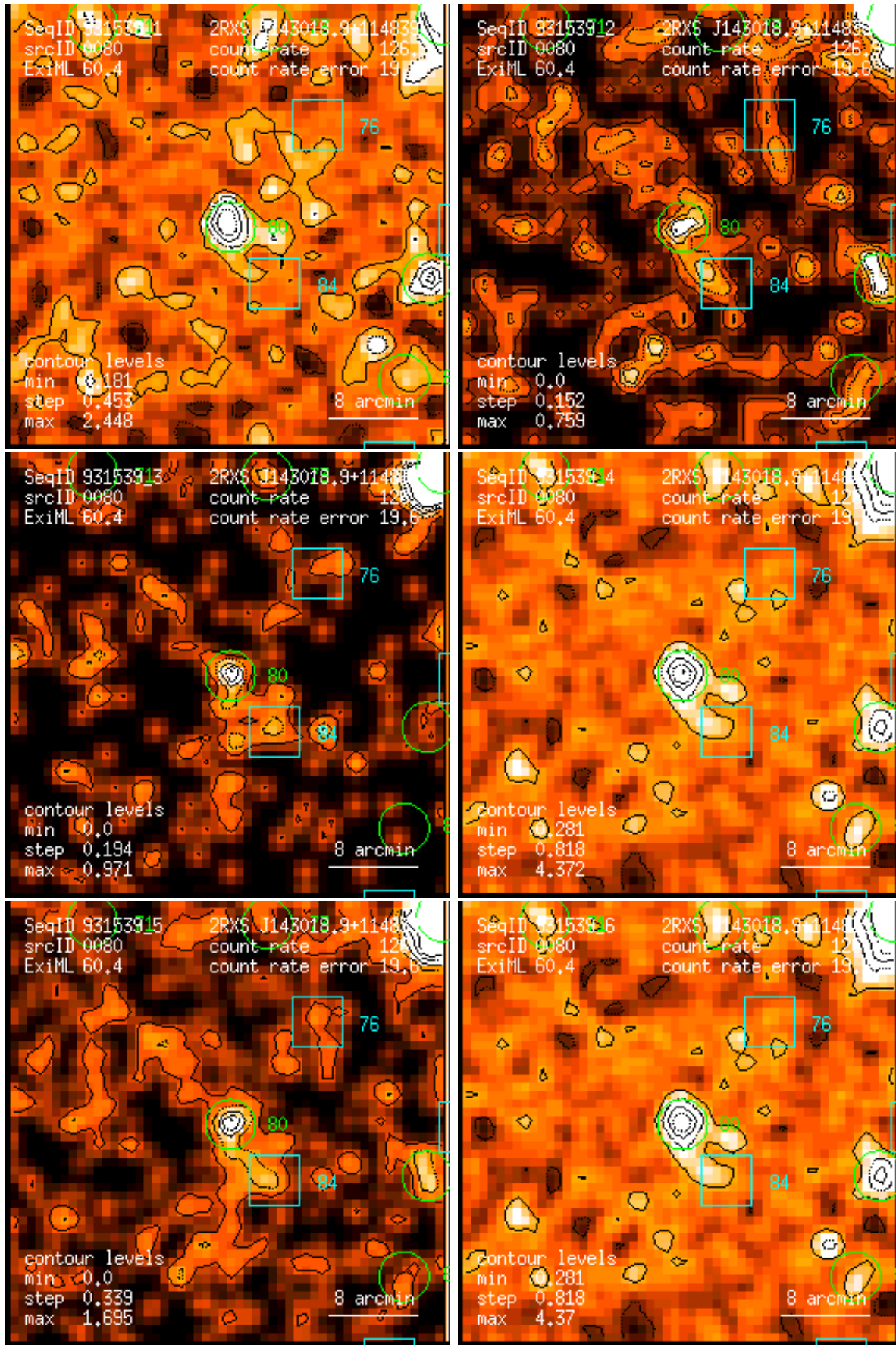
Figure 80: RASS 931539: detection 0080: band rate images, Gaussian filter: (1) PSPC channels 11 – 41, (2) 52 – 90, (3) 91 – 201, (4) 11 – 235, (5) 52 – 201, (6) 11 – 201. Broad band rates in counts/ks. Band rate contour levels in counts/ks/arcmin 2 .
