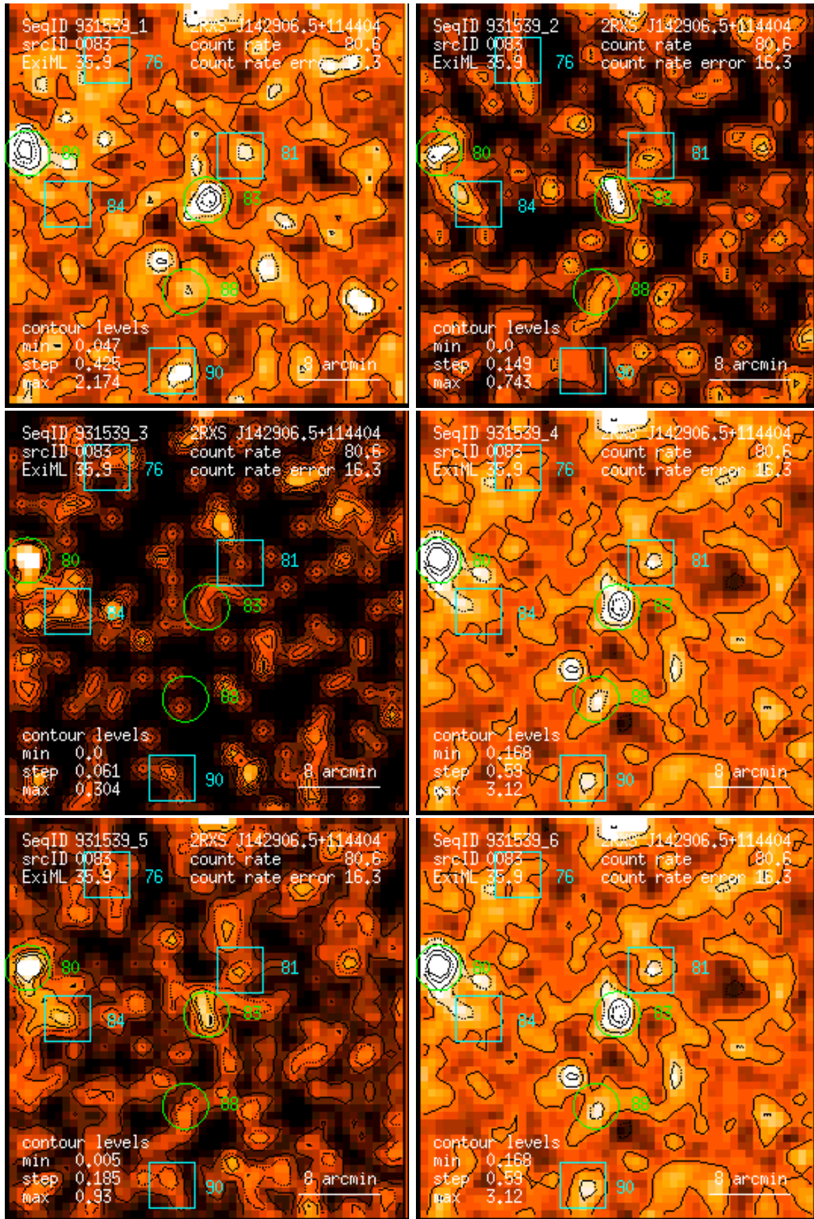
Figure 83: RASS 931539: detection 0083: band rate images, Gaussian filter: (1) PSPC channels 11 – 41, (2) 52 – 90, (3) 91 – 201, (4) 11 – 235, (5) 52 – 201, (6) 11 – 201. Broad band rates in counts/ks. Band rate contour levels in counts/ks/arcmin 2 .
