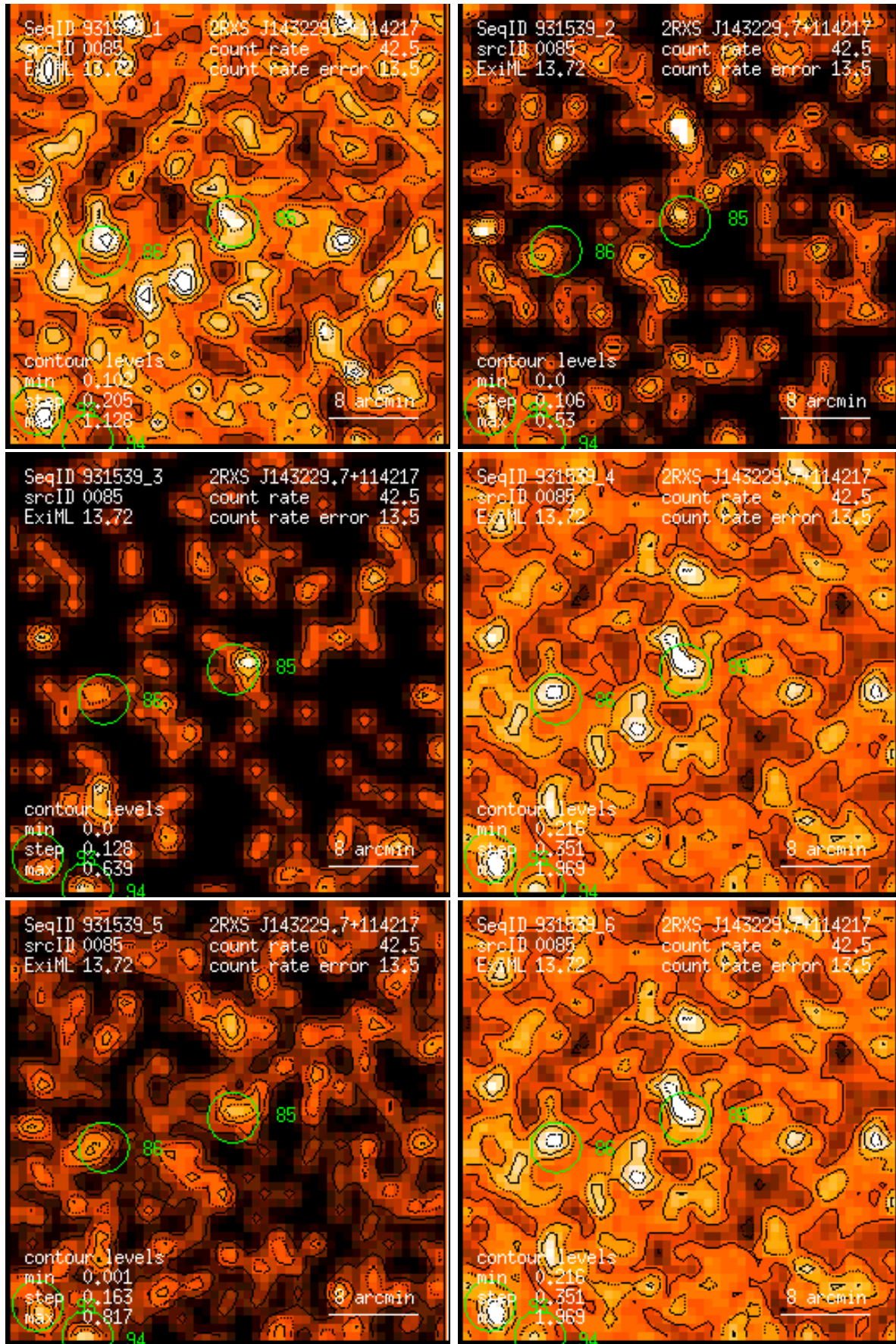
Figure 85: RASS 931539: detection 0085: band rate images, Gaussian filter: (1) PSPC channels 11 – 41, (2) 52 – 90, (3) 91 – 201, (4) 11 – 235, (5) 52 – 201, (6) 11 – 201. Broad band rates in counts/ks. Band rate contour levels in counts/ks/arcmin 2 .
