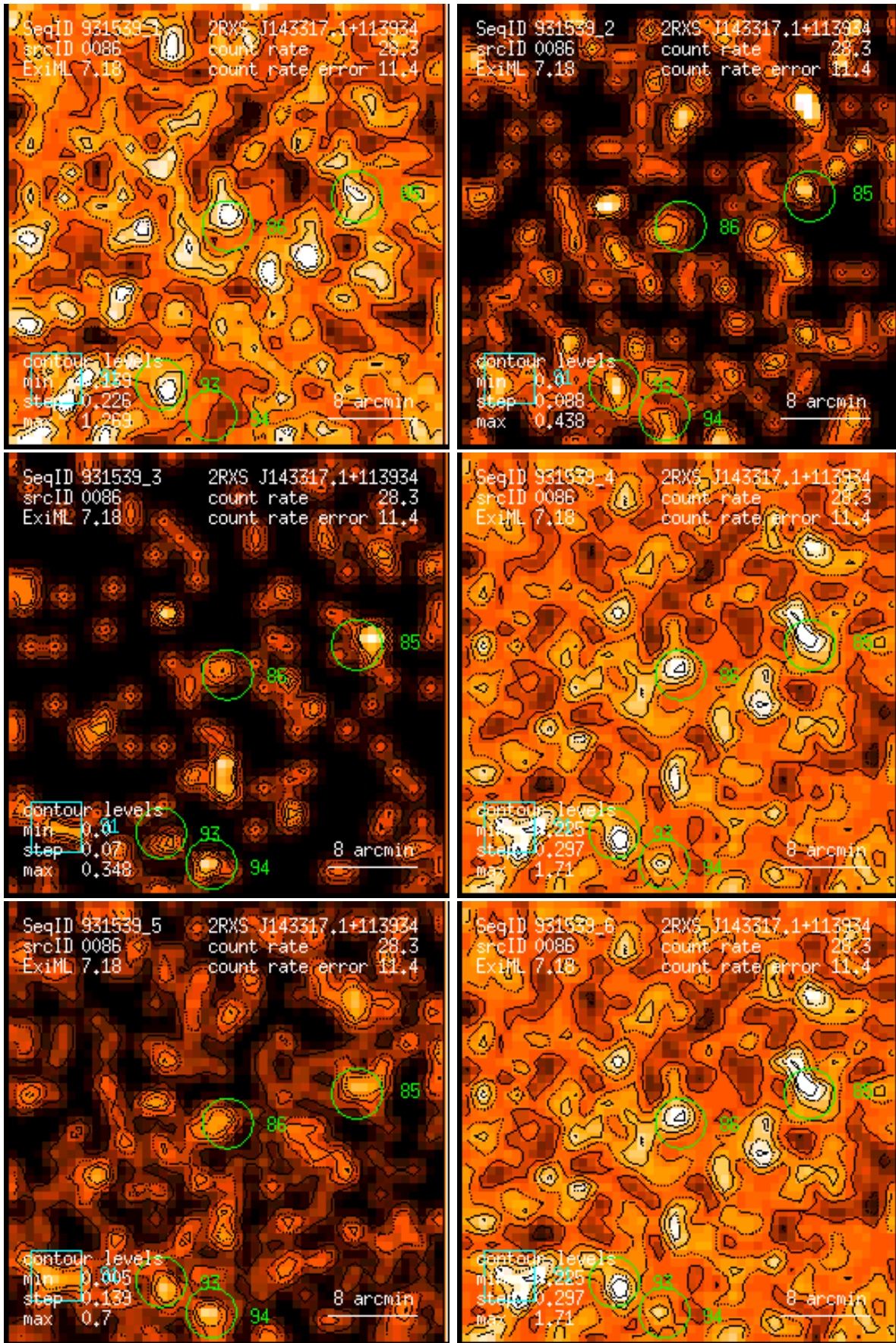
Figure 86: RASS 931539: detection 0086: band rate images, Gaussian filter: (1) PSPC channels 11 – 41, (2) 52 – 90, (3) 91 – 201, (4) 11 – 235, (5) 52 – 201, (6) 11 – 201. Broad band rates in counts/ks. Band rate contour levels in counts/ks/arcmin 2 .
