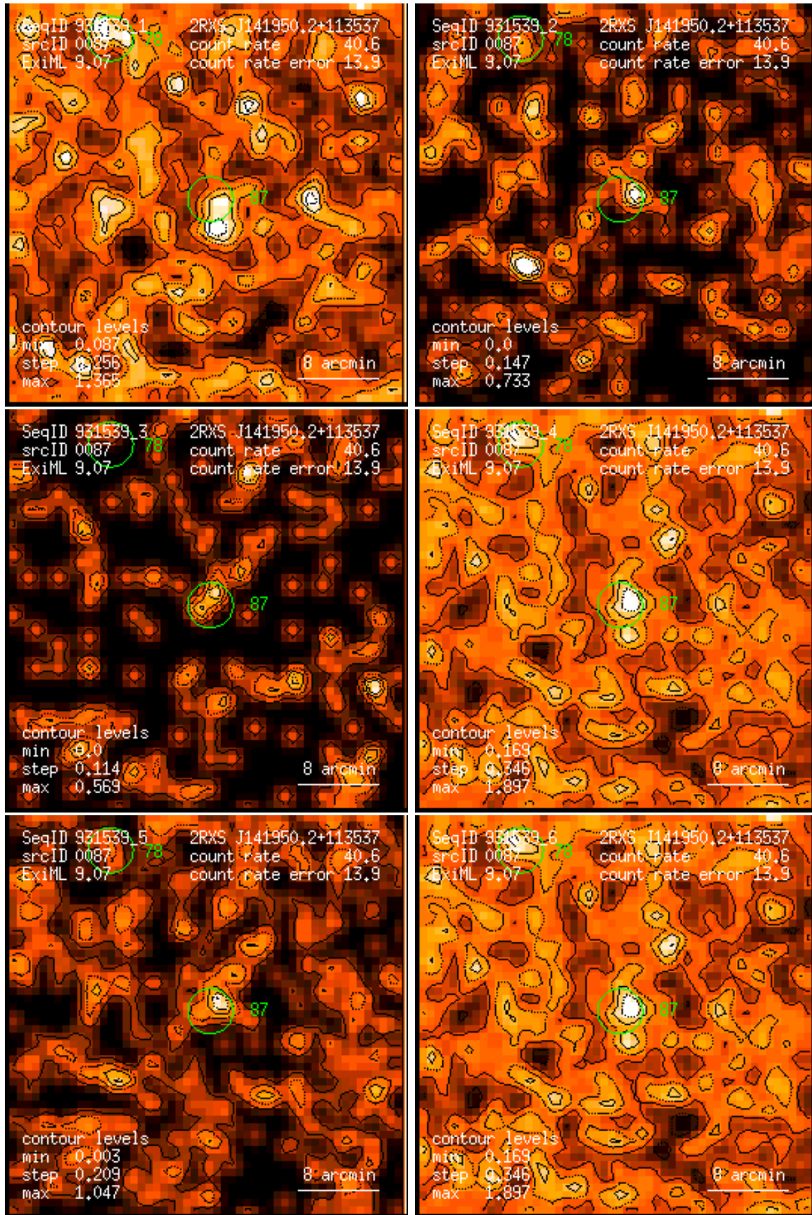
Figure 87: RASS 931539: detection 0087: band rate images, Gaussian filter: (1) PSPC channels 11 – 41, (2) 52 – 90, (3) 91 – 201, (4) 11 – 235, (5) 52 – 201, (6) 11 – 201. Broad band rates in counts/ks. Band rate contour levels in counts/ks/arcmin 2 .
