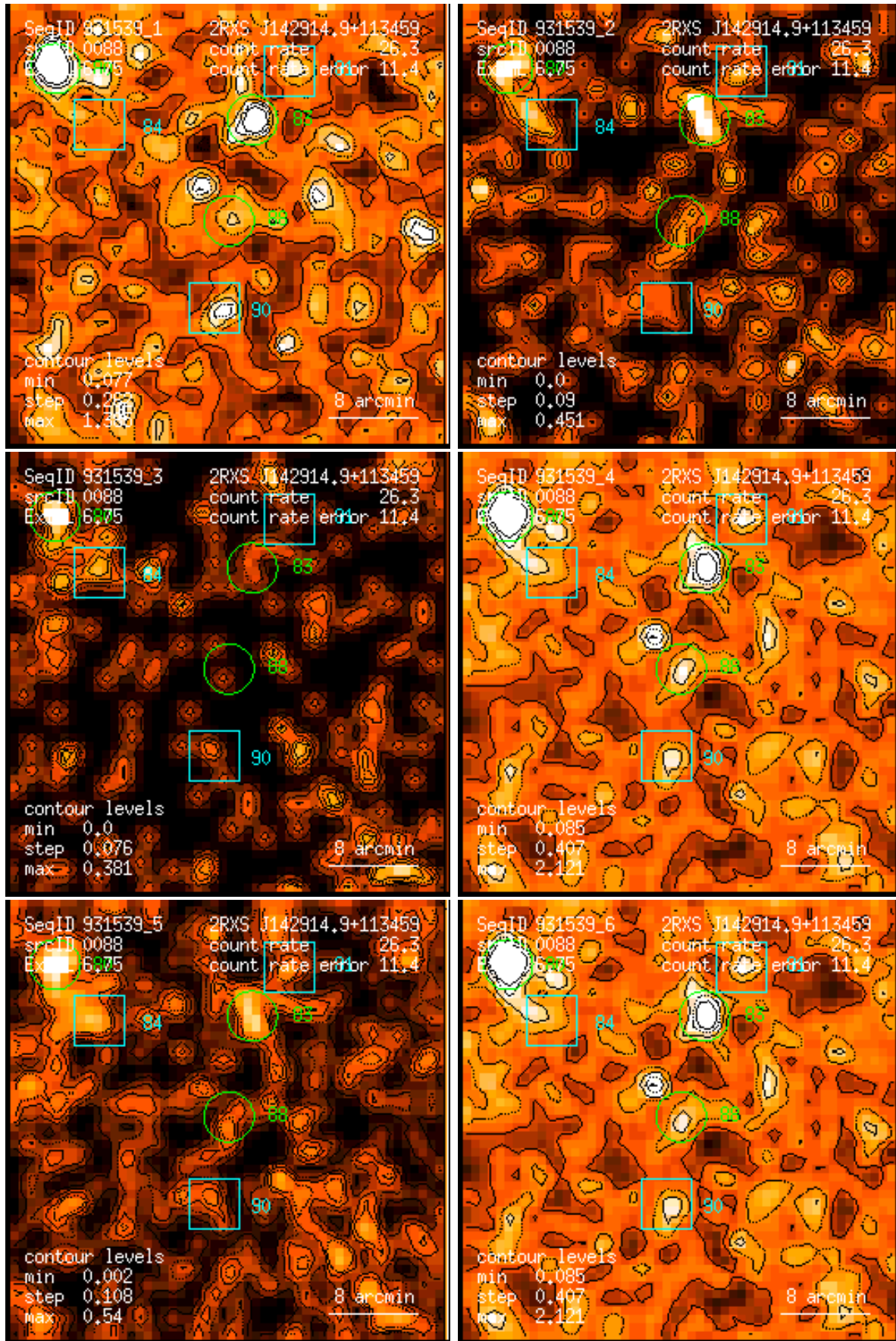
Figure 88: RASS 931539: detection 0088: band rate images, Gaussian filter: (1) PSPC channels 11 – 41, (2) 52 – 90, (3) 91 – 201, (4) 11 – 235, (5) 52 – 201, (6) 11 – 201. Broad band rates in counts/ks. Band rate contour levels in counts/ks/arcmin 2 .
