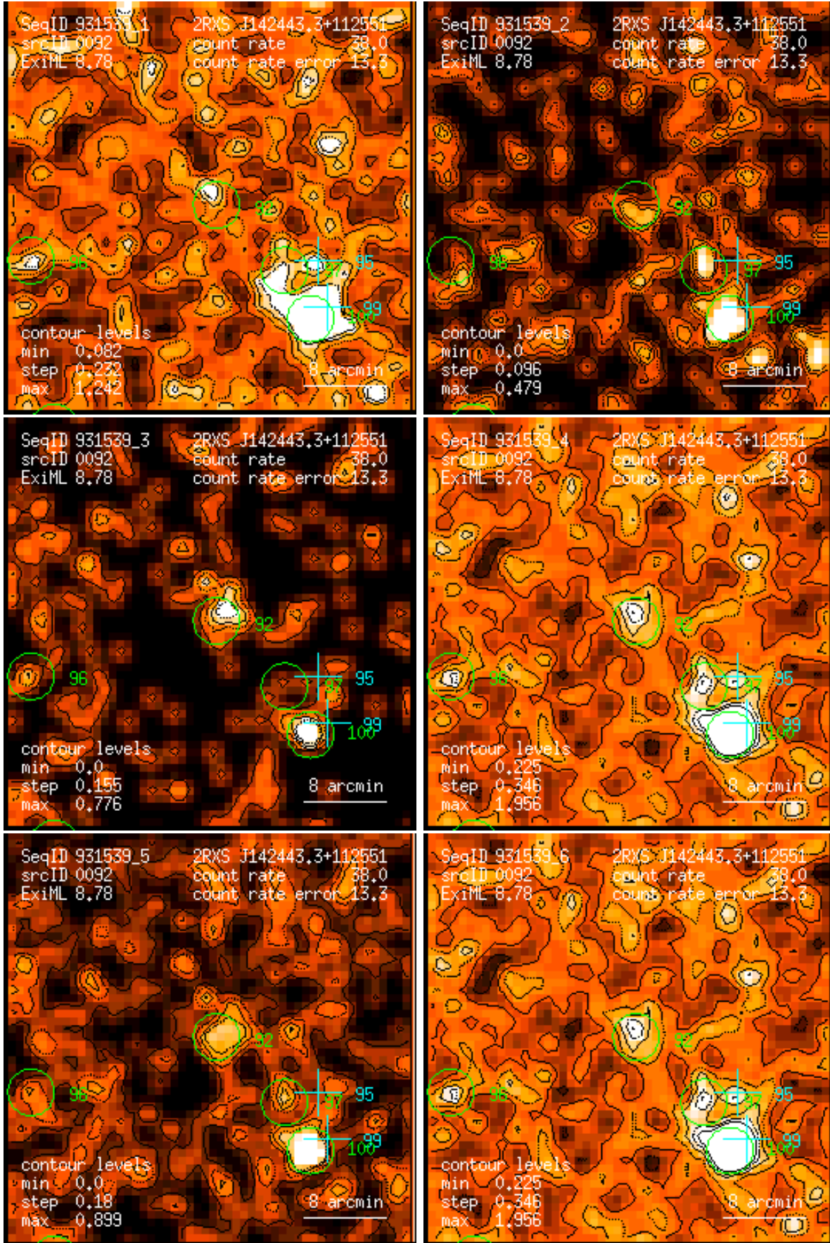
Figure 92: RASS 931539: detection 0092: band rate images, Gaussian filter: (1) PSPC channels 11 – 41, (2) 52 – 90, (3) 91 – 201, (4) 11 – 235, (5) 52 – 201, (6) 11 – 201. Broad band rates in counts/ks. Band rate contour levels in counts/ks/arcmin 2 .
