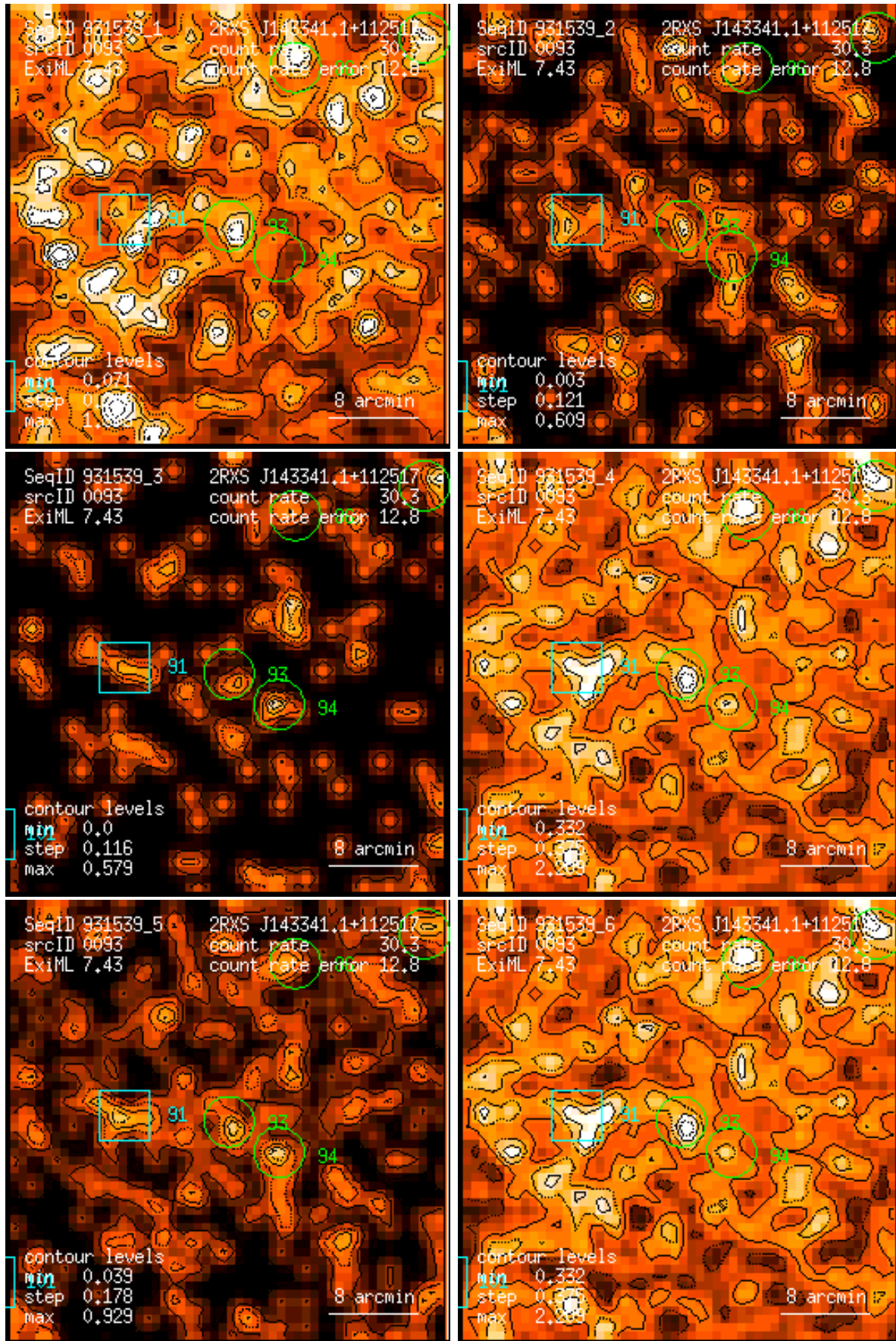
Figure 93: RASS 931539: detection 0093: band rate images, Gaussian filter: (1) PSPC channels 11 – 41, (2) 52 – 90, (3) 91 – 201, (4) 11 – 235, (5) 52 – 201, (6) 11 – 201. Broad band rates in counts/ks. Band rate contour levels in counts/ks/arcmin 2 .
