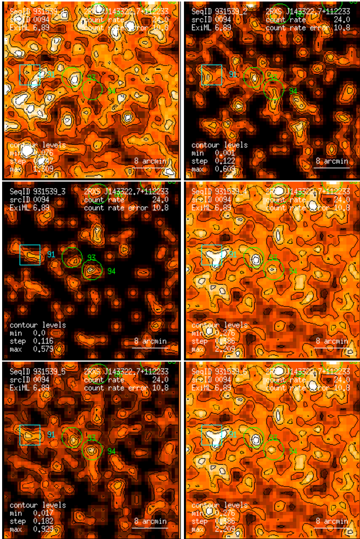
Figure 94: RASS 931539: detection 0094: band rate images, Gaussian filter: (1) PSPC channels 11 – 41, (2) 52 – 90, (3) 91 – 201, (4) 11 – 235, (5) 52 – 201, (6) 11 – 201. Broad band rates in counts/ks. Band rate contour levels in counts/ks/arcmin 2 .
