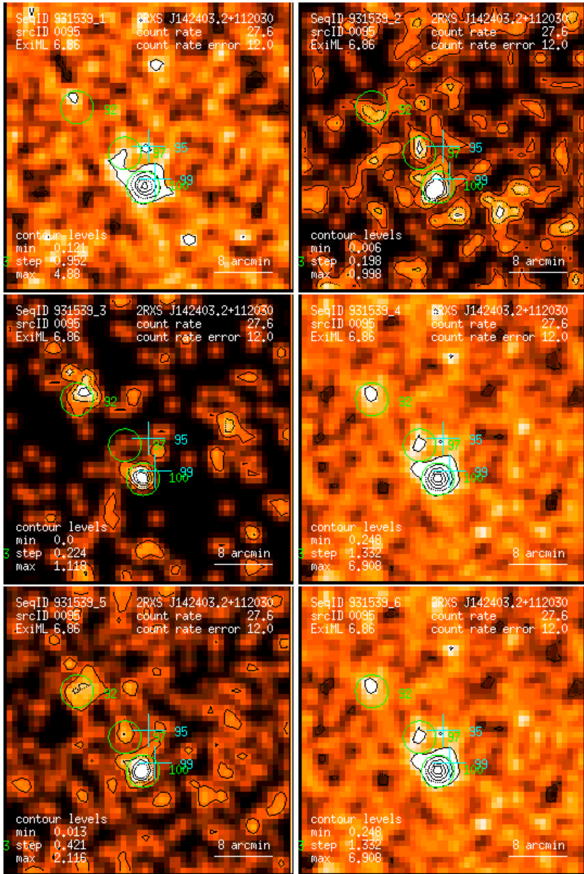
Figure 95: RASS 931539: detection 0095: band rate images, Gaussian filter: (1) PSPC channels 11 – 41, (2) 52 – 90, (3) 91 – 201, (4) 11 – 235, (5) 52 – 201, (6) 11 – 201. Broad band rates in counts/ks. Band rate contour levels in counts/ks/arcmin 2 .
