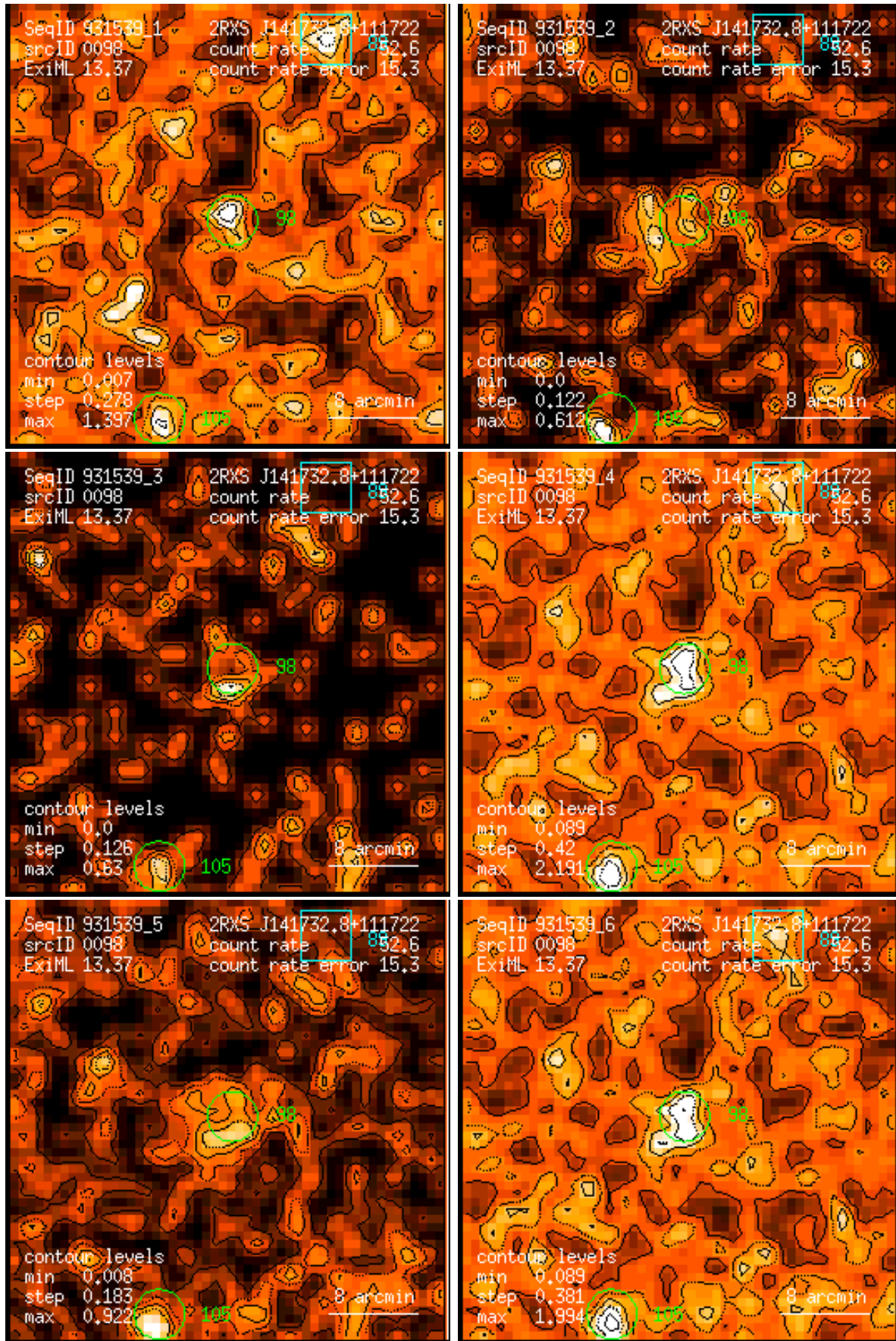
Figure 98: RASS 931539: detection 0098: band rate images, Gaussian filter: (1) PSPC channels 11 – 41, (2) 52 – 90, (3) 91 – 201, (4) 11 – 235, (5) 52 – 201, (6) 11 – 201. Broad band rates in counts/ks. Band rate contour levels in counts/ks/arcmin 2 .
