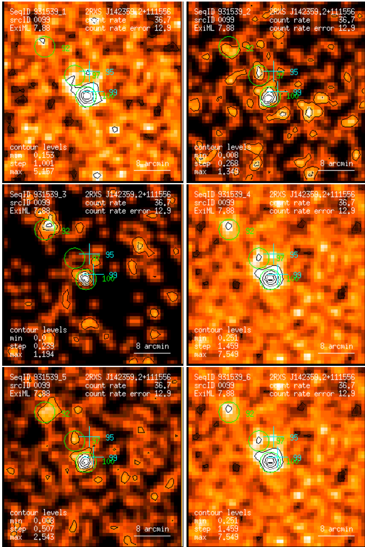
Figure 99: RASS 931539: detection 0099: band rate images, Gaussian filter: (1) PSPC channels 11 – 41, (2) 52 – 90, (3) 91 – 201, (4) 11 – 235, (5) 52 – 201, (6) 11 – 201. Broad band rates in counts/ks. Band rate contour levels in counts/ks/arcmin 2 .
