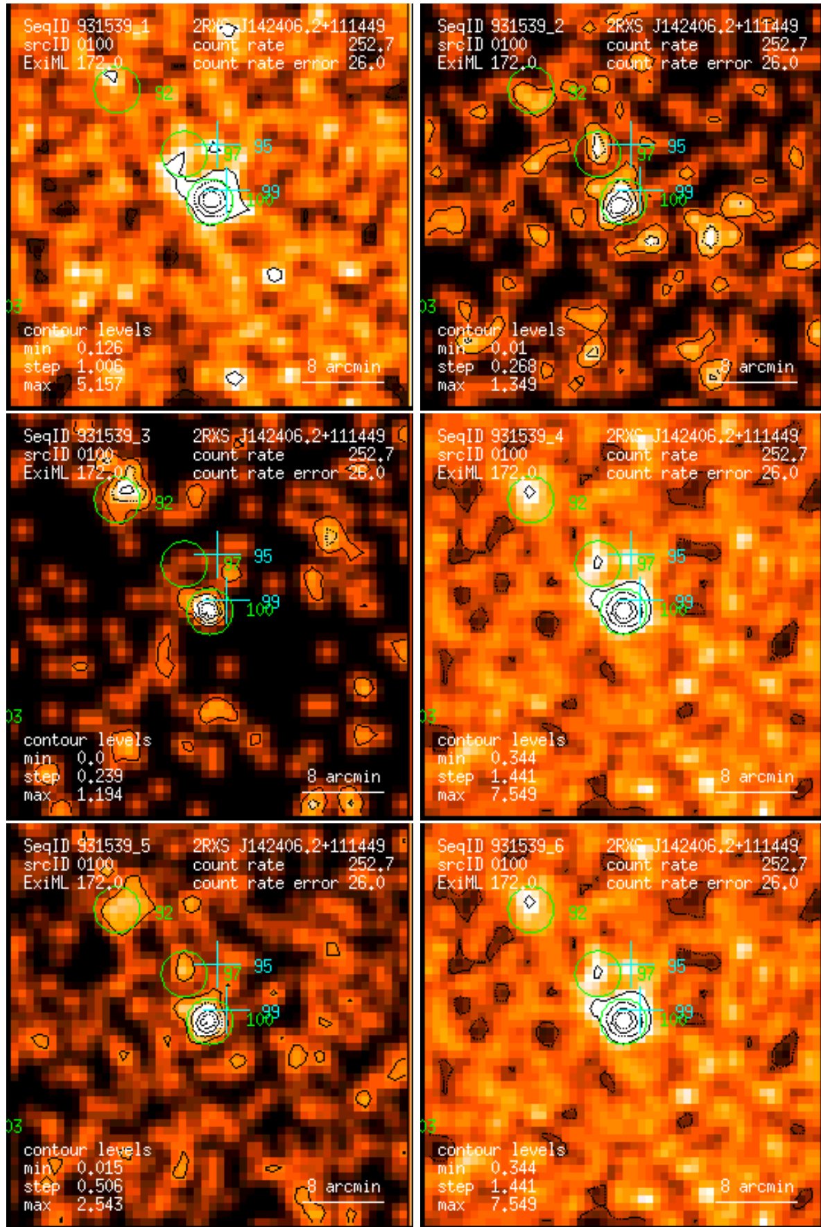
Figure 100: RASS 931539: detection 0100: band rate images, Gaussian filter: (1) PSPC channels 11 – 41, (2) 52 – 90, (3) 91 – 201, (4) 11 – 235, (5) 52 – 201, (6) 11 – 201. Broad band rates in counts/ks. Band rate contour levels in counts/ks/arcmin 2 .
