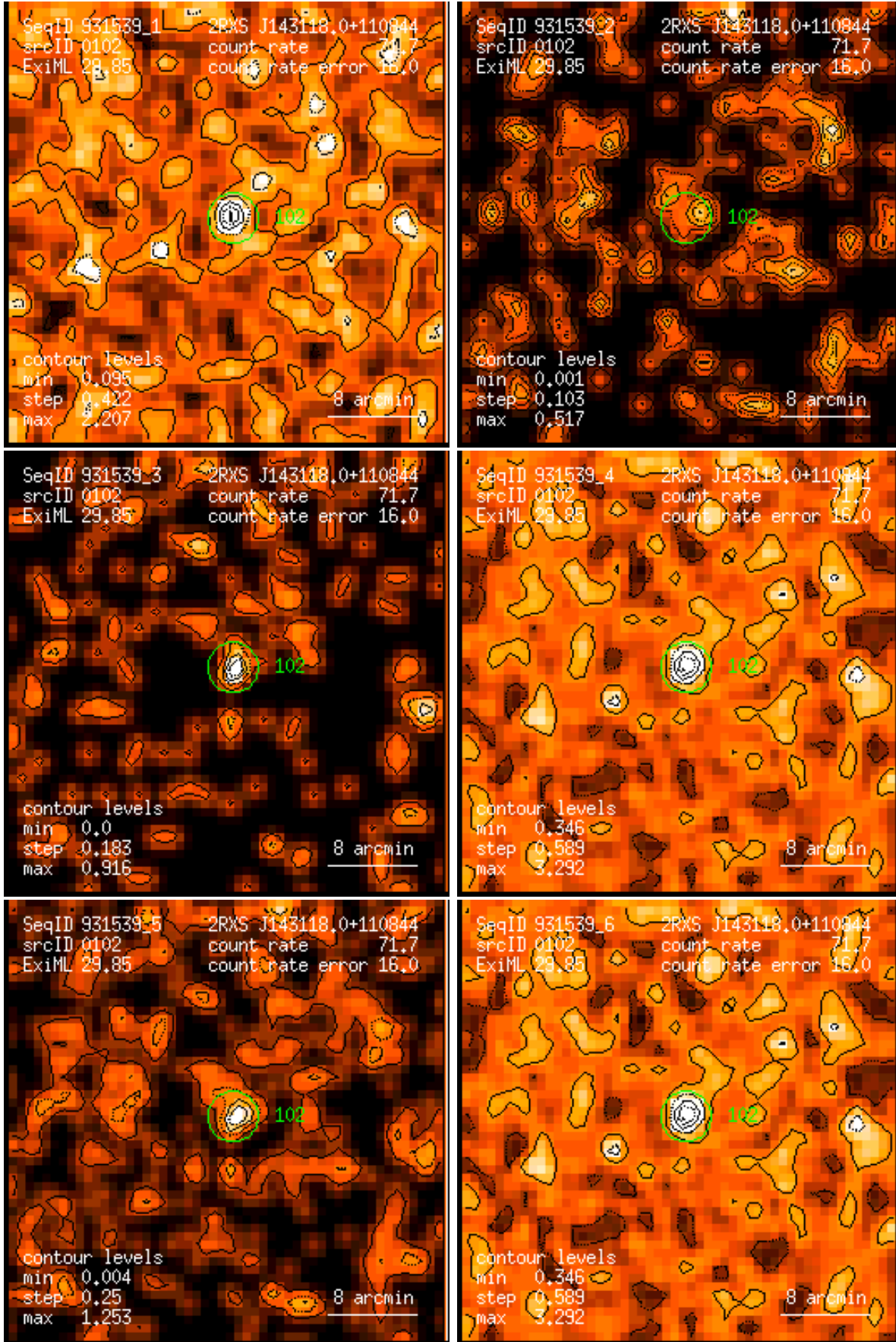
Figure 102: RASS 931539: detection 0102: band rate images, Gaussian filter: (1) PSPC channels 11 – 41, (2) 52 – 90, (3) 91 – 201, (4) 11 – 235, (5) 52 – 201, (6) 11 – 201. Broad band rates in counts/ks. Band rate contour levels in counts/ks/arcmin 2 .
