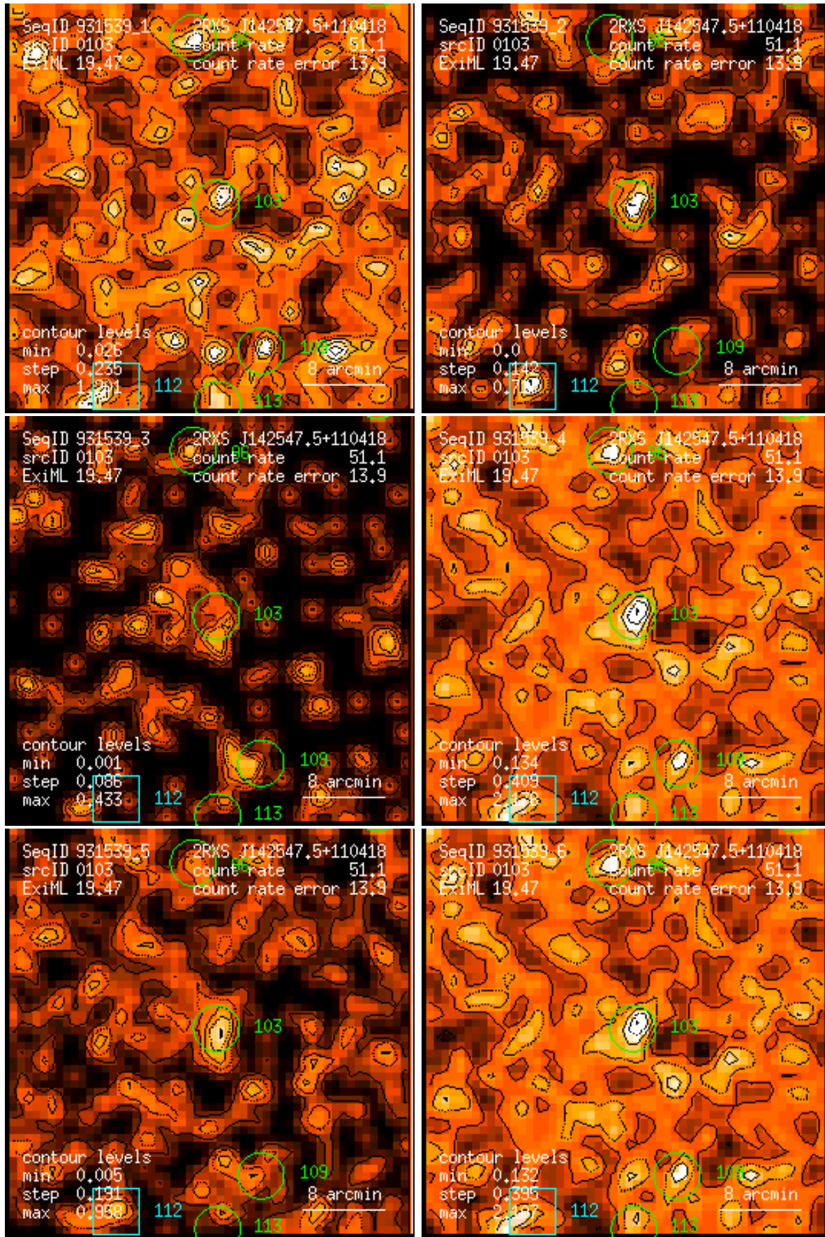
Figure 103: RASS 931539: detection 0103: band rate images, Gaussian filter: (1) PSPC channels 11 – 41, (2) 52 – 90, (3) 91 – 201, (4) 11 – 235, (5) 52 – 201, (6) 11 – 201. Broad band rates in counts/ks. Band rate contour levels in counts/ks/arcmin 2 .
