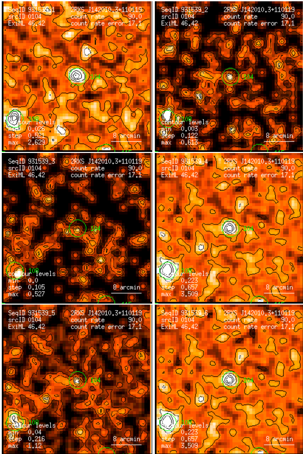
Figure 104: RASS 931539: detection 0104: band rate images, Gaussian filter: (1) PSPC channels 11 – 41, (2) 52 – 90, (3) 91 – 201, (4) 11 – 235, (5) 52 – 201, (6) 11 – 201. Broad band rates in counts/ks. Band rate contour levels in counts/ks/arcmin 2 .
