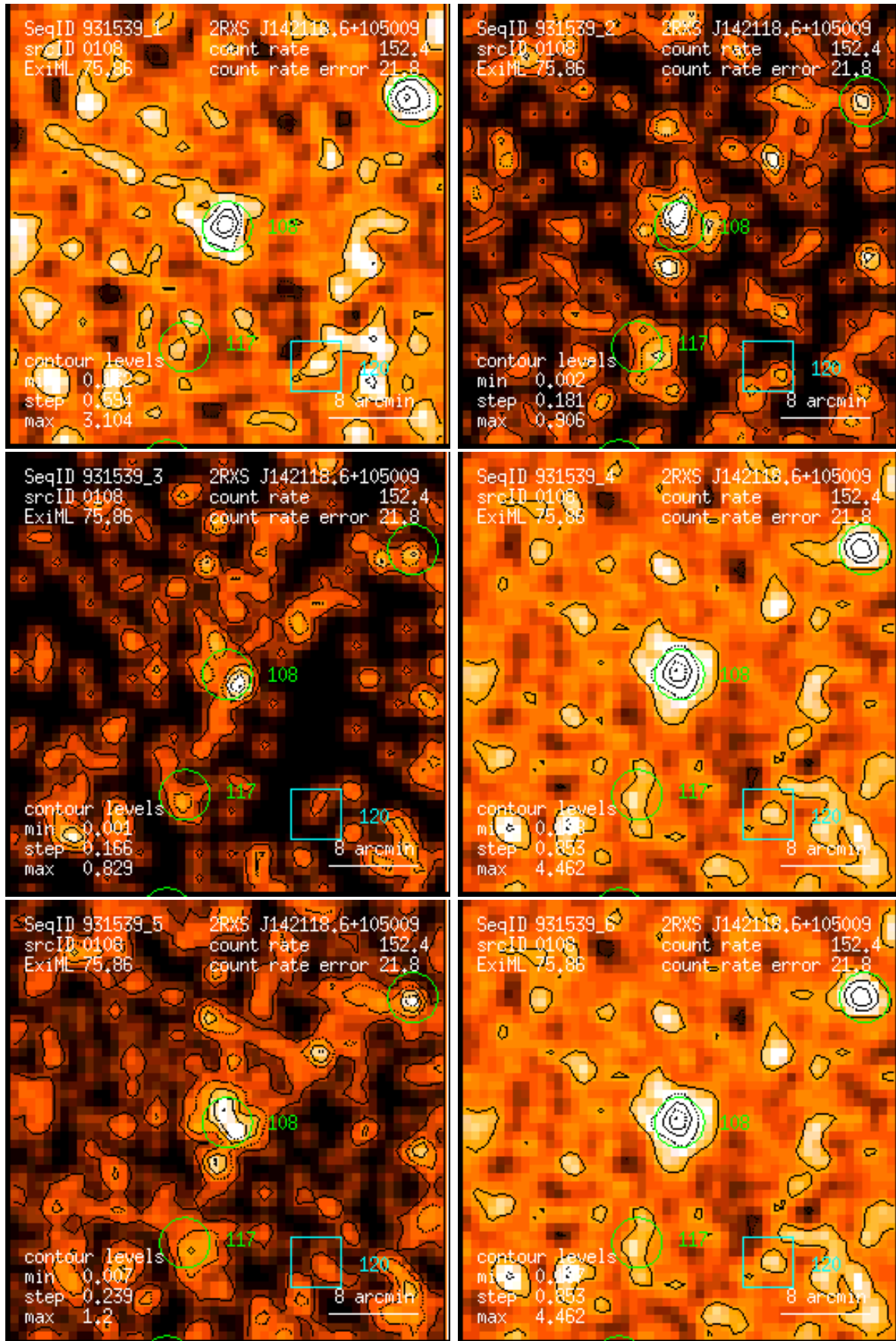
Figure 108: RASS 931539: detection 0108: band rate images, Gaussian filter: (1) PSPC channels 11 – 41, (2) 52 – 90, (3) 91 – 201, (4) 11 – 235, (5) 52 – 201, (6) 11 – 201. Broad band rates in counts/ks. Band rate contour levels in counts/ks/arcmin 2 .
