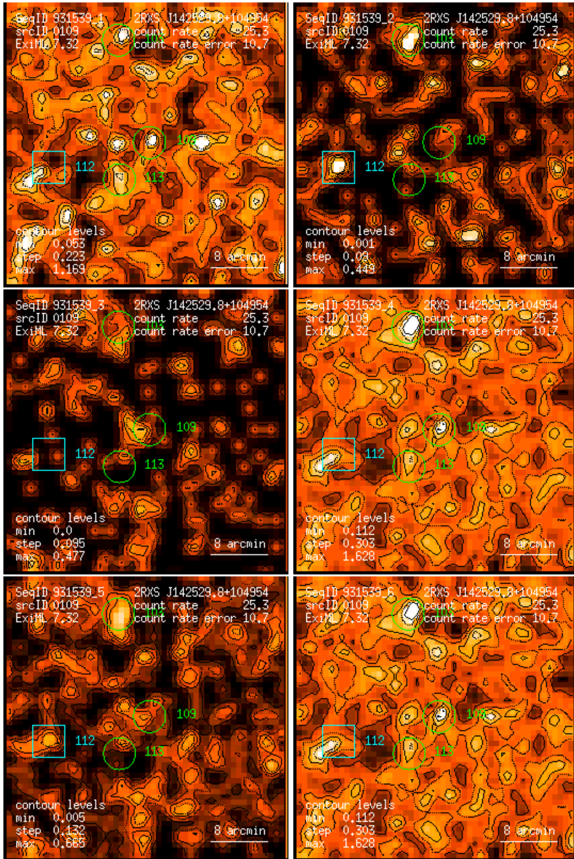
Figure 109: RASS 931539: detection 0109: band rate images, Gaussian filter: (1) PSPC channels 11 – 41, (2) 52 – 90, (3) 91 – 201, (4) 11 – 235, (5) 52 – 201, (6) 11 – 201. Broad band rates in counts/ks. Band rate contour levels in counts/ks/arcmin 2 .
