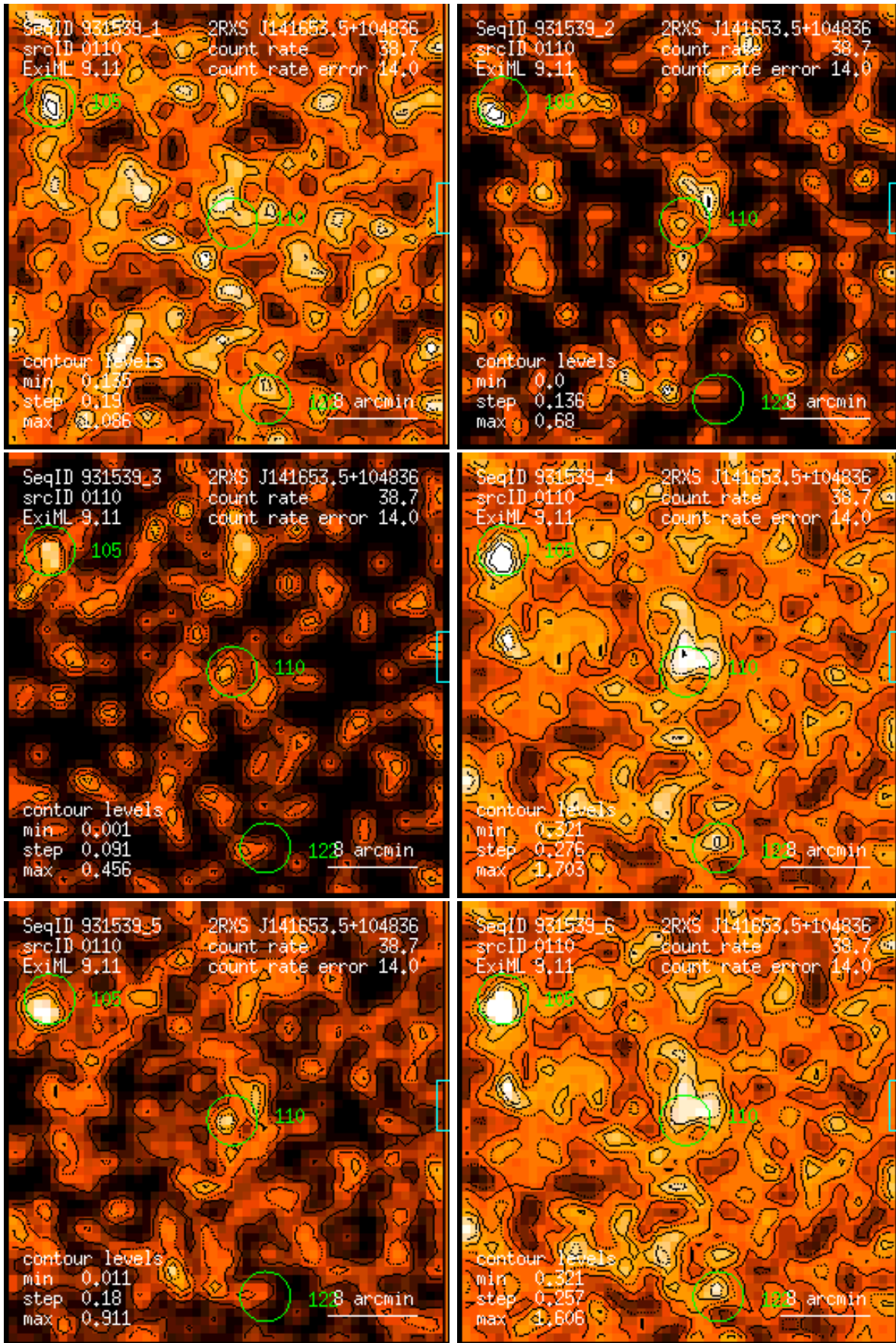
Figure 110: RASS 931539: detection 0110: band rate images, Gaussian filter: (1) PSPC channels 11 – 41, (2) 52 – 90, (3) 91 – 201, (4) 11 – 235, (5) 52 – 201, (6) 11 – 201. Broad band rates in counts/ks. Band rate contour levels in counts/ks/arcmin 2 .
