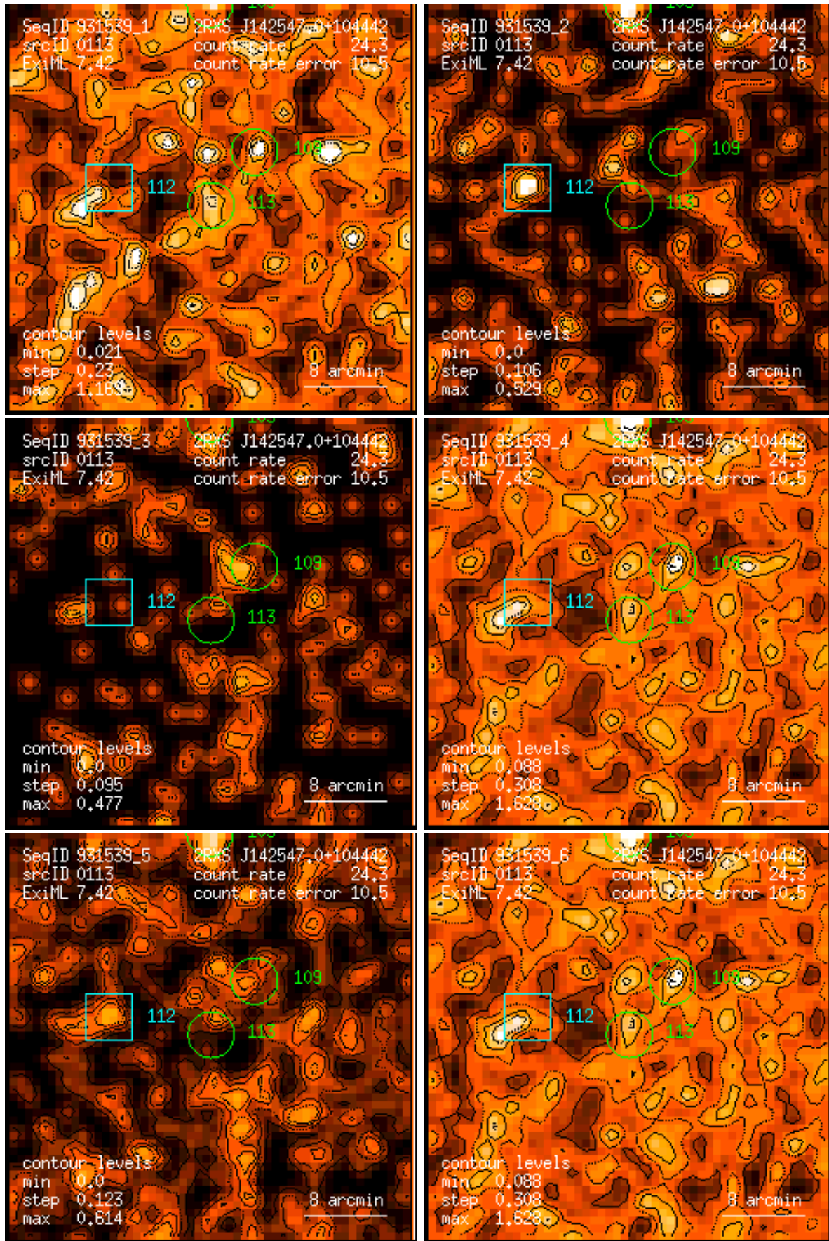
Figure 113: RASS 931539: detection 0113: band rate images, Gaussian filter: (1) PSPC channels 11 – 41, (2) 52 – 90, (3) 91 – 201, (4) 11 – 235, (5) 52 – 201, (6) 11 – 201. Broad band rates in counts/ks. Band rate contour levels in counts/ks/arcmin 2 .
